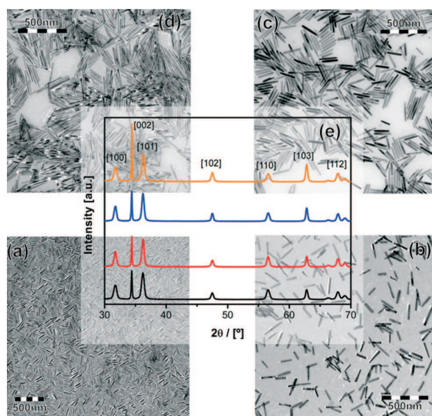
Fig. 2 TEM (a d) and PXRD data (e) of samples prepared for continuous addition of ZnO precursor (a; black graph \leftrightarrow a; red graph \leftrightarrow b; blue graph \leftrightarrow c; orange graph \leftrightarrow d).
