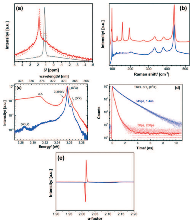
Fig. 3 Spectroscopic investigation of LZO nanorods ( red) in comparison to ZO nanorods ( blue): (a) ^7\text{Li} solid state NMR spectra of LZO rods (prior \cong dotted line, after purification \cong solid line) and lithium stearate ( grey line) as reference. (b) Raman spectra taken at room temperature. (c) PL spectra taken at T = 5\text{ K} . Both spectra are normalized to neutral donor bound exciton luminescence at 3.3567\text{ eV} ( I_0 ). (d) TRPL of I_0 ( D^0X ). (e) X band EPR spectra.
