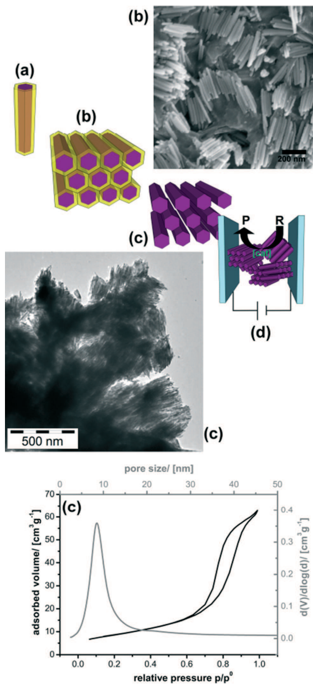
Fig. 5 Oriented attachment (b; SEM data and schematic image) of single LZO nanorods (a). The porous nanorod material obtained after calcination (c; TEM data, nitrogen physisorption data and pore size distribution function and schematic image). Device architecture for testing the materials in chemical sensing (d).
