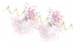
Figure 8. Model of H-AP 10 C(Gd-PyMTA)P 10 C(Gd-PyMTA)P 10 -NH 2 (peptide 9 ) with the conformation of a right-handed PPI helix. Chosen dihedral angles for modeling: \phi = -75^\circ , \psi = 160^\circ and \omega = 0^\circ . The calculated rotamer conformations are displayed via the opaque clouds.
