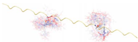
Figure 6. Model of H-AP 10 C(Gd-PyMTA)P 10 C(Gd-PyMTA)P 10 -NH 2 (peptide 9 ) with the conformation of a polyproline type II helix with the common dihedral angles of: \phi = -75^\circ , \psi = 145^\circ , and \omega = 180^\circ . The calculated rotamer conformations are displayed via the opaque clouds.
