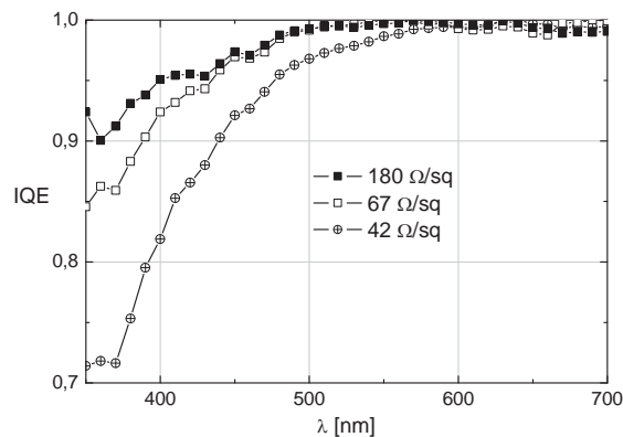
Figure 8: Blue response of 50 \times 50 \text{ mm}^2 selective emitter solar cells with 10 \Omega/\square sheet resistance under the grid lines and different sheet resistance in the illuminated areas.
