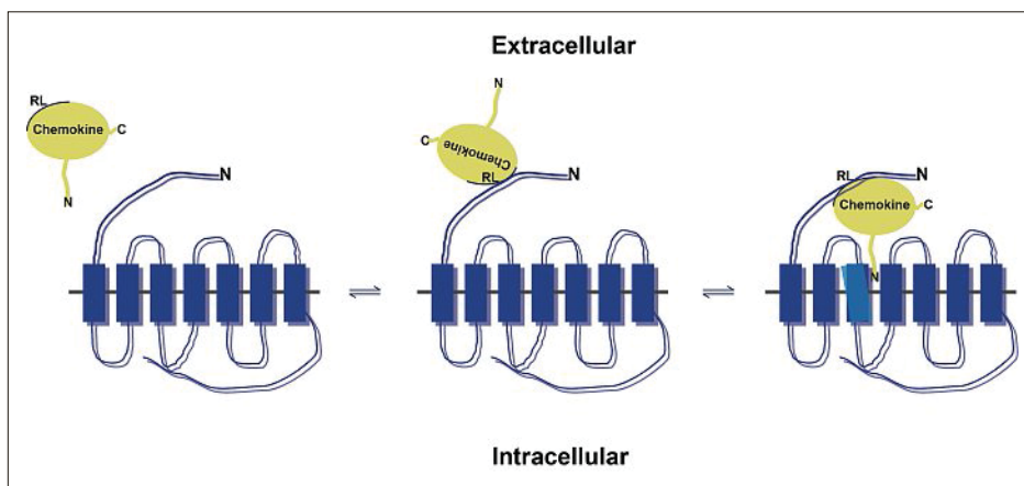
Fig. 2. Two-step chemokine receptor binding model. Chemokines (in yellow) first dock to the N-terminus of the heptahelical receptor via their rigid loop (RL). Subsequently, the N-terminus of the chemokine falls into the binding pocket embedded in the transmembrane helices leading to receptor conformational changes (indicated in light blue) and receptor activation. N-termini (N), C-termini (C). Figure adapted from Crump et al. [5]
