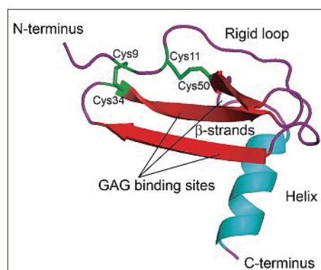
Fig. 1. Chemokine fold and structural features. Monomeric human CXCL12 [22-93] X-ray structure (PDBe Monomer_3GV).
