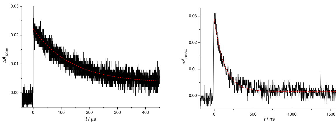
Figure S9: Laser flash spectra and decaying curves (at 420 nm and 600 nm) of T5S0-O(CO)Thy in nitrogen saturated MeOH. Solutions were adjusted to an absorbance of 0.215 at 355 nm, the excitation wavelength.
