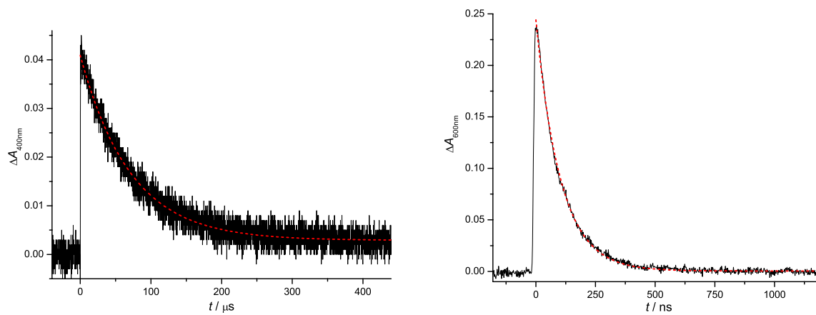
Figure S3: Laser flash spectra and decaying curves (at 400 nm and 600 nm) of T7S4-O(CO)Thy in nitrogen saturated MeOH. Solutions were adjusted to an absorbance of 0.215 at 355 nm, the excitation wavelength.
