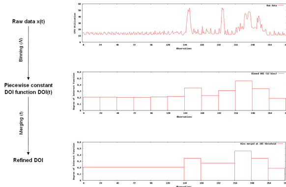
Figure 5: DOI extraction from raw time series by determining the interestingness score over the time series for a number of bins N , followed by (optional) merging of bins with similar interestingness scores.
