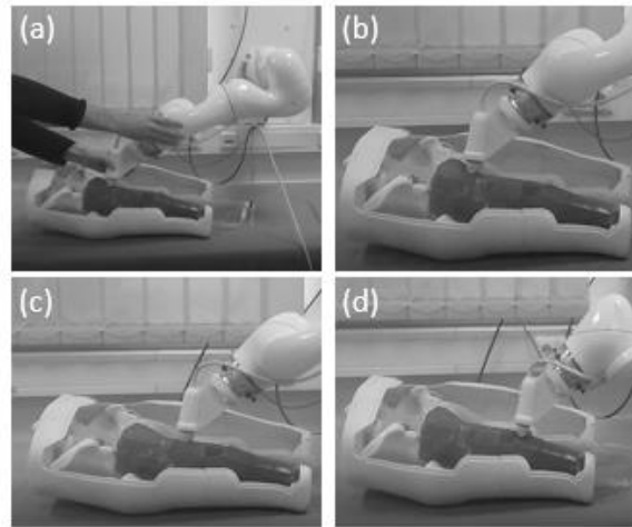
Figure 3: (a) The hand guidance mode allows to place the US probe on the leg phantom. (b)-(d) The robot arm moves along the leg, the artery center always in the horizontal center of the US image.
