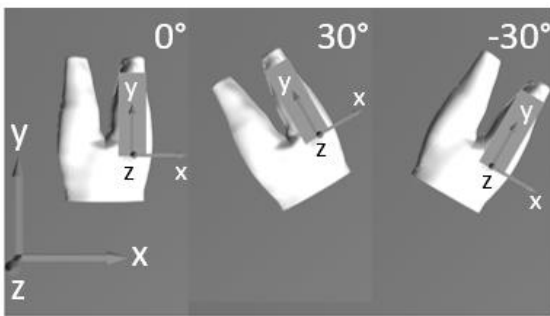
Figure 2: The world coordinate system (bottom left) and the end effector coordinate system after placing the US probe using the hand guidance mode for each rotation of the phantom. Note that the z-axes of both systems are always identical.
