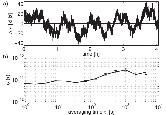
FIG. 4. (a) Measurement of the beat signal \nu_{b2} between the 10 GHz and the 1 GHz comb over 4 h. The graph gives the offset from the average value of 837.1856 MHz. (b) Corresponding Allan deviation with error bars for the frequency measurement.
