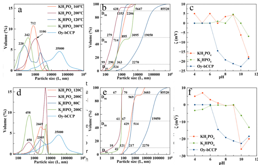
Fig. 5 Volume based CSD (a) and (d), cumulative volume based CSD (b) and (e), and \zeta potential versus pH (c) (f) of Oy-bCCP and HA particles prepared at different temperatures using \text{KH}_2\text{PO}_4 and \text{K}_2\text{HPO}_4 and P/bCCP molar ratios of 0.6 (a) (c), and 0.96 (d) (f). Note that CSDs of HA and Oy-bCCP particles, though plotted in the same figures, were measured by different techniques, i.e., DLS and laser diffraction, respectively.
