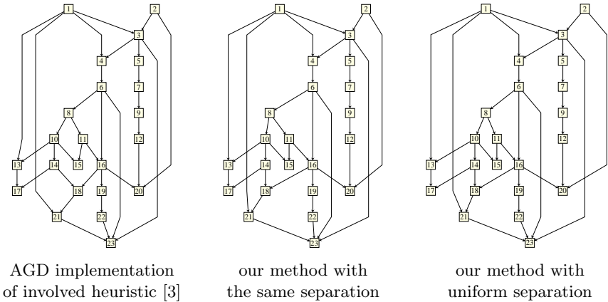
Fig. 4. Final assignments compared
