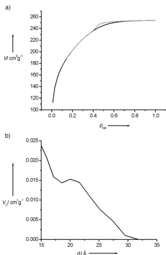
Figure 2. \text{N}_2 isotherm of \gamma -HPCD-silica (a, adsorption printed in black, desorption in gray) and the corresponding DFT pore size distribution (b). V = adsorbed volume, p_{\text{rel}} = relative pressure, V_D = differential pore volume, d = diameter.
