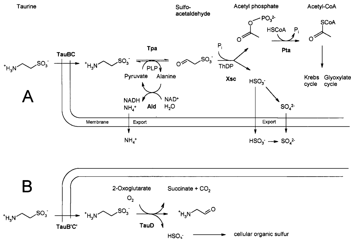
Fig. 1. Pathway of dissimilation of taurine in R. opacus ISO-5 with putative homeostatic mechanisms to detoxify sulfite and maintain the osmolarity in the cell (A), and dioxygenolytic desulfonation of taurine to aminoacetaldehyde for the assimilation of taurine sulfur (B). Different transport systems are inferred for the high fluxes involved in supplying carbon and nitrogen from taurine for growth (A), compared with the low flux and high affinity required to supply sulfur from taurine (B). Abbreviations not used in the Introduction: PLP, pyridoxal 5'-phosphate; ThDP, thiamin diphosphate.
