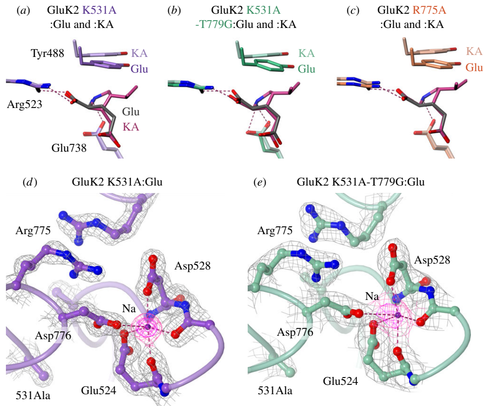
Figure 3. Ligand-binding cleft and dimer-interface interactions in GluK2 mutant LBD structures. (a) Simplified view of the ligand-binding sites in K531A:Glu (purple) and K531A:KA (light purple). Glu and KA are shown grey and magenta, respectively. Side chains directly interacting with ligand (R523 and E738; magenta dashes indicate H bonds) are shown, along with Y488, which is shifted upwards in the KA complex. (b,c) Equivalent views for K531A-T779G:Glu and :KA (green and pale green) and R775A:Glu and :KA (orange and pale orange). (d) Region around protomer B cation binding site in K531A:Glu, viewed from 'above' the LBD dimer (approx. 35° from the twofold axis). Key side chains and main chain atoms are shown as ball-and-stick. Contacts with the sodium ion (purple sphere) are indicated by magenta dashes. Electron density, (2F_{\text{obs}} - F_{\text{calc}})\alpha_{\text{calc}} , is shown around the displayed residues (grey mesh; contoured at 1.5 \sigma ), and sodium (magenta mesh; contoured at 1.5 \sigma and 3.0 \sigma ). (e) View of K531A-T779G:Glu, displayed as in (d).
