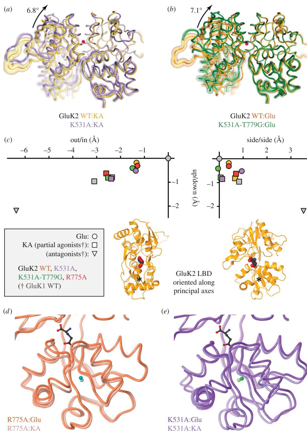
Figure 5. Domain movements in apical GluK2 mutants. (a) Comparison of D1:D1 dimer conformation in WT:KA and K531A:KA structures. Cartoons show averaged C\alpha coordinates determined following alignment to the D1 domain of GluK2 WT protomer A. Variability is indicated by tube diameter (transparent overlay where >0.4 Å; see §3). Structures are viewed down the axis for D1:D1 movement (magenta dot; magnitude of rotation indicated). (b) Equivalent view comparing WT:Glu and K531A-T779G:Glu. (c) Movement of D2 domain centres of mass along principal axes showing correlations with ligand efficacy. The left graph shows ‘cleft closure’ (i.e. up/down and in/out movement) and the right graph ‘twist’ (up/down and side/side). The orange cartoons illustrate the protomer orientation for the graphs above (asterisk marks D2 centre of mass). Points (see boxed key) are plotted relative to the 3_{FUZ} GluK1 WT:Glu complex (grey circle). For GluK1 structures, the points are average movements from selected structures of partial agonists (AHCP, 2WKY; KA, 3c32; Dom, 2PBW) and antagonists (ATPO, 1vso; UBP310, 2oIT; a thiophene derivative, 3s2v). Efficacy is correlated with both cleft closure (left graph) and sideways shifts (right graph). (d) Cartoon of R775A:Glu and :KA LBD (averaged C\alpha coordinates), aligned on the D1 domain. The D2 domain of the Glu complex is shifted up and to the right compared with the KA complex (see centres of mass, indicated by dark and light cyan spheres). (e) Equivalent view comparing K531A:Glu and :KA, showing reversal of sideways shift in this mutant.
