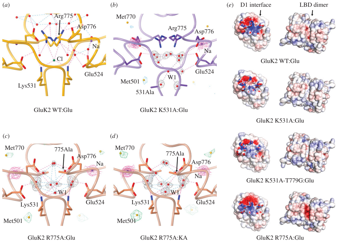
Figure 4. The anion binding pocket in GluK2 K531A and R775A mutants. (a) Ion binding sites in WT:Glu LBD structure (PDB code 2xrr), viewed perpendicular to the dimer twofold. \text{Na}^+ and \text{Cl}^- ions (purple and green, respectively) are shown, along with key side chains and interacting waters. (b) Equivalent view for K531A:Glu. Electron density, (2F_{\text{obs}} - F_{\text{calc}})\alpha_{\text{calc}} is shown around the sodium ions (magenta mesh, 1.5\sigma and 4.0\sigma ) and waters (grey mesh, 1.5\sigma ) only. Anomalous difference-Fourier electron density (green mesh, 3.5\sigma ) is also shown. Clear anomalous-difference peaks are observed at buried methionine sulphur atoms (M501, yellow spheres), with weaker peaks at surface sulphurs (M770). W1 indicates the modelled water closest to the chloride site, but no significant (greater than 2.5\sigma ) anomalous difference peaks were associated with this or any other solvent molecule in the vicinity. (c,d) Equivalent views for the R775A:Glu and R775A:KA complexes, with anomalous difference-Fourier electron density contoured at 4.0\sigma . Density modelled as solvents (W1) was present near the usual chloride ion binding site, but, again, no significant anomalous difference peaks were present. (e) Electrostatic surface potential calculated for the dimeric LBD in the absence of ions. Images on the left show the D1 interface on protomer A (red = -10 k_B T/e ; blue = +10 k_B T/e ), whereas images on the right show the intact LBD dimer viewed from 'above' ( -8 to +8 k_B T/e ). Distinct binding sites for sodium (red; both views) and chloride (blue; interface view) are visible in the GluK2-WT:Glu complex, as described previously [11,12]. The sodium binding site is still present in the mutants, but the chloride binding site is either poorly defined (K531A-containing mutants), or partly masked by more negative surface electrostatics (R775A mutant).
