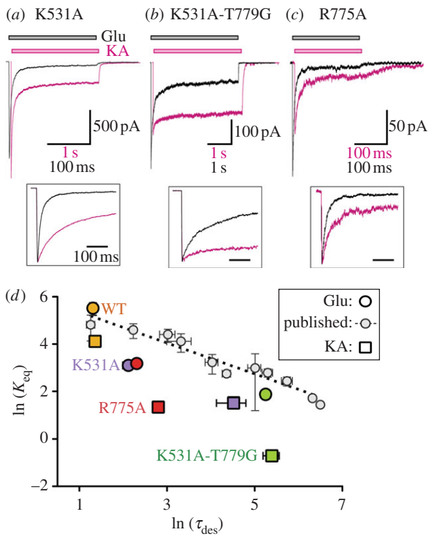
Figure 2. Functional effects of K531A, K531A-T779G and R775A mutations on GluK2 responses to Glu and KA. (a) Responses to applications of 10 mM Glu (400 ms; black trace) and 1 mM KA (4 s; magenta trace), recorded from outside-out patches pulled from HEK cells transfected with K531A. The traces are shown on a different time-base and horizontally offset to allow easier comparison of relative efficacy and steady-state responses. The inset shows the same traces on an equal time-base and with normalized peak heights, to allow comparison of desensitization rates. (b,c) Traces recorded in response to Glu and KA applications (7 s in (b); 0.4 s in (c)) from cells transfected with K531A-T779G and R775A respectively (displayed as in (a)). (d) Graph comparing the steady-state equilibrium constant ( K_{eq} ) with the first-order desensitization time constant ( \tau_1 ). Values are plotted as the natural logarithm (mean \pm s.e.m.), making them proportional to free-energy of desensitization ( \Delta G_{des} ) and activation energy ( E_a or \Delta G^{++} ), respectively. The dotted line is the linear regression ( r^2 = 0.94 ) through data points (small light grey circles; ‘published’) calculated from steady-state and desensitization-rate data for the ten GluK2 mutants plus WT described by Chaudhry et al. [10].
