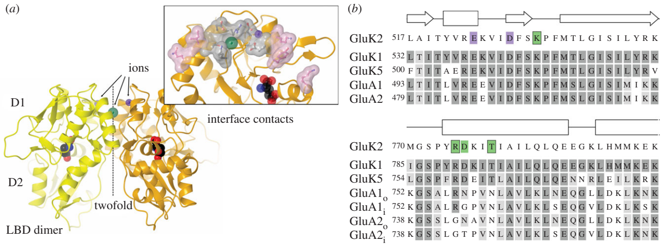
Figure 1. Apical interactions within GluK2 LBD dimer. (a) The GluK2 WT LBD dimer (PDB code 2XXR) [7] showing ligand (black), domains D1 and D2, the twofold axis and the \text{Na}^+ and \text{Cl}^- ions (purple and green, respectively). Key D1:D1 interactions are shown inset on protomer B; pink surface from data in reference [8] and grey surface from this study. (b) Sequence alignment for kainate (GluK1, 2 and 5) and AMPA (GluA1 and 2; i and o indicate flip and flop splice variants). GluA2 is shown edited at the R/G site (743). Dark grey shading shows identity and light grey conserved. Secondary structure (from GluK2) is indicated by rectangles ( \alpha -helices) and arrows ( \beta -strands). GluK2 residues involved in the cation and anion binding sites are highlighted in purple and green, respectively (mutated residues are boxed).
