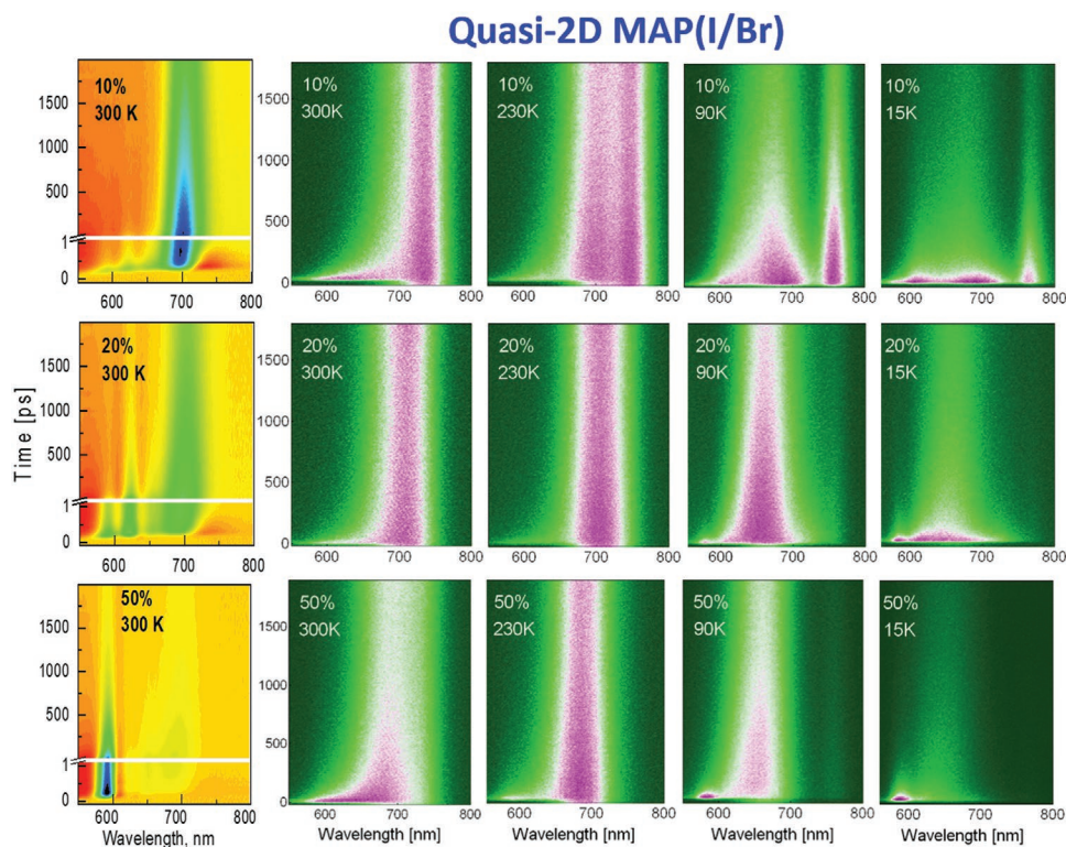
Figure 4. TA evolution for quasi-2D MAPI 2 Br 1 samples with 10%, 20%, and 50% BA contents at room temperature and PL evolutions at different temperatures.
