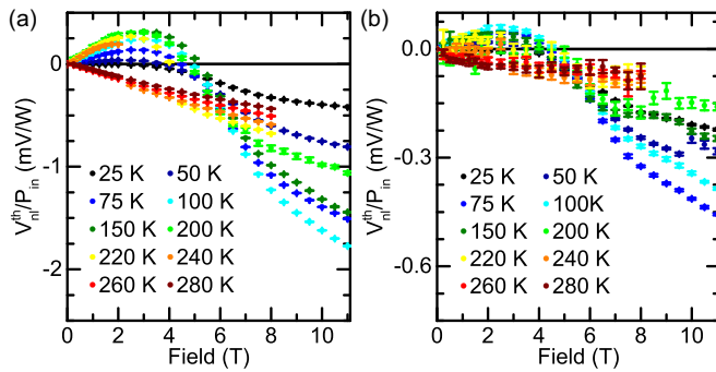
FIG. 7. Nonlocal spin Seebeck signal parallel to the in-plane projection of the easy-axis in hematite for a magnetic field applied parallel to the transport direction across a distance of (a) 500 nm or (b) 7\ \mu\text{m} . The magnitude of \mathbf{H} stated is that along x . The general shape and trends are identical between the two distances. The error bars represent the standard deviation of the data point.
