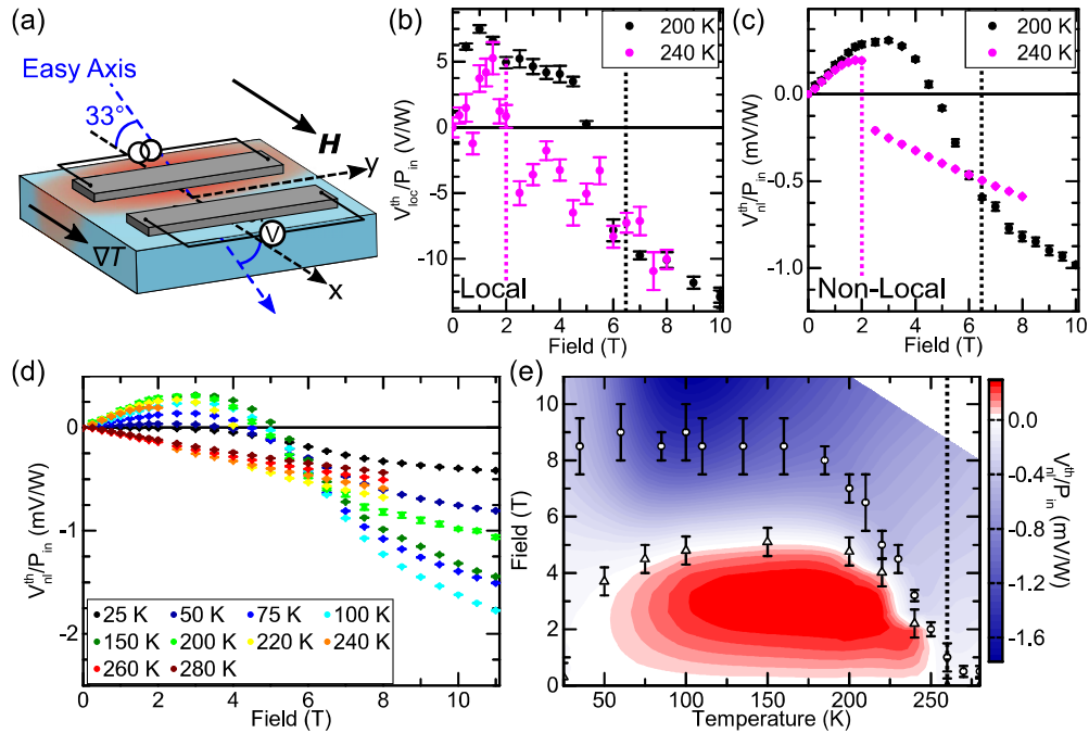
FIG. 2. (a) Geometry used to investigate the nonlocal spin Seebeck effect (NL-SSE) in hematite (blue). A passing charge current heats the hematite below one Pt wire, generating a thermal gradient \nabla T . The easy-axis is inclined at 33^\circ to the surface plane and a magnetic field \mathbf{H} is applied parallel in the in-plane component of the Néel vector. (b) Local SSE as a function of magnetic field at T = 240 K (magenta) and T = 200 K (black). The dashed line indicates the spin-flop field at the respective temperature. (c) NL-SSE at T = 240 K (magenta) and T = 200 K (black) as a function of the applied magnetic field. The dashed lines indicate the spin-flop field at the respective temperature. (d) NL-SSE as a function of the applied magnetic field parallel to the in-plane component of the easy-axis for temperatures above and below the Morin transition temperature ( T_M = 257 K). (e) NL-SSE as a function of field and temperature. Open circles indicate the spin-flop field from Ref. [28] and triangles indicate the inversion field from panel (d). The dashed line indicates T_M . The magnitude of \mathbf{H} stated is that along x .
