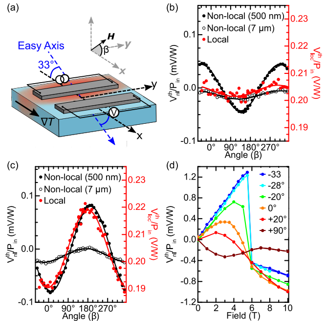
FIG. 8. (a) Nonlocal geometry for investigating the nonlocal spin Seebeck effect in hematite for transport parallel to the in-plane projection of the easy-axis. The magnetic field is applied at an angle \beta as indicated where \beta = 0^\circ occurs for \mathbf{H} parallel to x . (b) Local (red, right axis) and nonlocal (black closed and open symbols, left axis) spin Seebeck signals at 200 K under a magnetic field of \mu_0\mathbf{H} = 2\ \text{T} rotated through an angle \beta . The solid lines represent fits to a \sin \beta function. (c) Local (red, right axis) and nonlocal (black closed and open symbols, left axis) spin Seebeck signals at 200 K under a magnetic field of \mu_0\mathbf{H} = 8\ \text{T} rotated through an angle \beta . The solid lines represent fits to a \sin \beta function. (d) Nonlocal spin Seebeck signal for a fixed value of \beta for a wire separation of 500 nm at 200 K.
