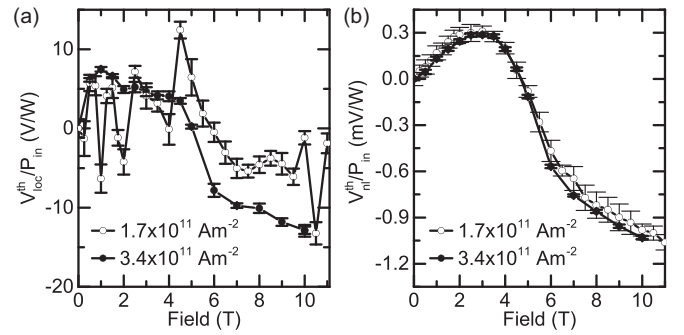
FIG. 6. (a) Local spin Seebeck effect measured for the geometry in Fig. 2(a) as a function of the applied magnetic field for two current densities. (b) nonlocal spin Seebeck effect measured for the geometry in Fig. 2(a) as a function of the applied magnetic field for two current densities. Error bars represent the standard deviation of the data point.
