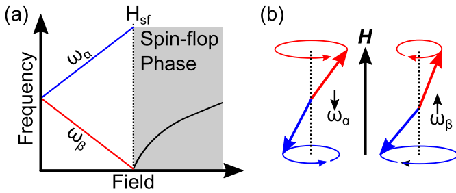
FIG. 1. (a) Schematic magnon dispersion as a function of an applied field for a uniaxial antiferromagnet. The application of a magnetic field splits the degeneracy of the two lowest magnon modes. At the spin-flop field H_{sf} , the frequency of one mode reaches zero and the two circular modes change character. (b) Schematic of the two easy-axis modes. The right circularly polarized mode \omega_\alpha and the left circularly polarized mode \omega_\beta .
