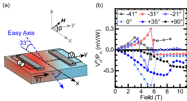
FIG. 9. (a) Nonlocal geometry for investigating the nonlocal spin Seebeck effect in hematite for transport perpendicular to the in-plane projection of the easy-axis. The magnetic field is applied at an angle \beta as indicated where \beta = 0^\circ occurs for \mathbf{H} parallel to \mathbf{x} . (b) Nonlocal spin Seebeck signal for a fixed value of \beta for a wire separation of 500 nm at 200 K and a current density of 2 \times 10^{11} A m ^{-2} .
