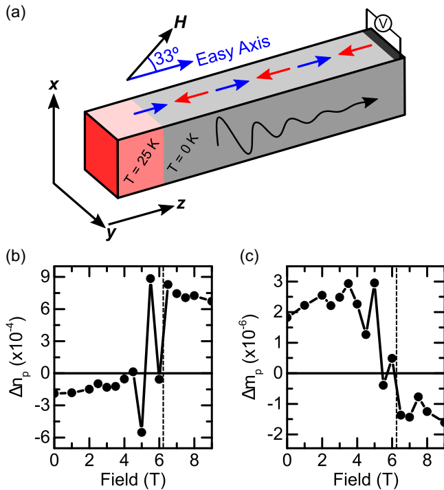
FIG. 4. (a) Geometry used for calculations with a size N_x \times N_y \times N_z = 16 \times 16 \times 12288 . A temperature step of 25 K was used to excite the magnetic ordering and we probe the perturbation from equilibrium of the Néel vector and magnetization some distance from this excitation. The easy-axis is aligned along the transport direction and a magnetic field \mathbf{H} is applied at 33^\circ to the easy-axis. (b) Perturbation of the Néel vector from equilibrium ( \mathbf{n}_0 ) as a function of the applied field, projected along the magnetic field, where \Delta n_p is defined in the main text. (c) Perturbation of the magnetization from equilibrium ( \mathbf{m}_0 ) as a function of the applied field, projected along the magnetic field, where \Delta m_p is defined in the main text. The dashed lines indicates the spin-flop field of the system.
