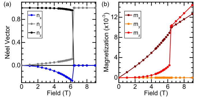
FIG. 5. (a) x , y , and z components of the Néel vector under an applied magnetic field at 33^\circ to the easy-axis for our choice of parameters. We find the spin-flop to occur at \mu_0\mathbf{H} = 6.4\text{T} , similar to the experimental observation. (b) x , y , and z components of the magnetization under an applied magnetic field for our choice of parameters. Above the spin-flop field, a large component of \mathbf{m} appears parallel to the field.
