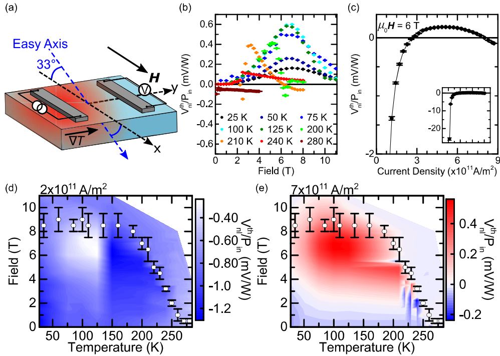
FIG. 3. (a) Nonlocal schematic for wires parallel to x . The magnetic field is parallel to the easy-axis in-plane projection and perpendicular to the thermal gradient \nabla T . (b) Nonlocal antiferromagnetic spin Seebeck effect as a function of field for temperatures below T_M . The magnitude of \mathbf{H} stated is that along x . (c) Current dependence of the nonlocal signal normalized to the input power. The inset shows the same data but on a larger y -axis due to the divergent behavior at low input currents (d, e) Phase diagram of the nonlocal spin Seebeck signal as a function of field and temperature for two current densities, 2 \times 10^{11} \text{ A m}^{-2} and 7 \times 10^{11} \text{ A m}^{-2} respectively. The circles represent the spin-flop field taken from Ref. [28].
