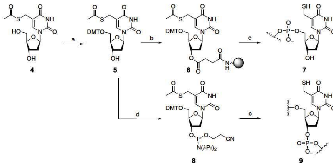
Scheme 2. Synthesis of DNA oligonucleotides containing 5-(mercaptomethyl) 2'-deoxyuridines. Reagents and conditions: (a) DMT Cl, DMAP, pyridine, 0 °C, 24 h, (90%); (b) EDC, DMAP, succinylated LCAA CPG, pyridine; then 4 nitrophenol; then piperidine, then acetic anhydride/pyridine/THF (cap A) and 1 methylimidazole/THF (cap B); (c) i) oligonucleotide synthesis, ii) DBU, then 33% NH 4 OH, 0.2 M DTT; (d) [( i -Pr) 2 N](NCCH 2 CH 2 O)PjCl, NEt 3 , CH 2 Cl 2 , rt, 4 h, (66%).
