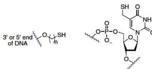
Figure 1. Thioalkyl functions conjugated to the 5' or 3' end of DNA (left), 5 (mercaptomethyl) 2' deoxyuridine moieties incorporated into DNA oligonucleotides.
