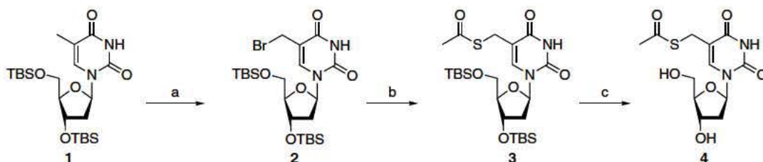
Scheme 1. Synthesis of 5-(mercaptomethyl) 2'-deoxyuridine. Reagents and conditions: (a) NBS, AIBN, CCl 4 , reflux, 2.5 h; (b) potassium thioacetate, DMF, 1.5 h, (39%, over two steps); (c) AcOH, THF, 24 h (73%).
