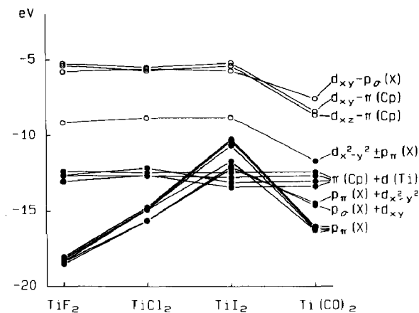
Fig. 2. Orbital energy diagram for filled (●) and empty (○) MOs calculated for \text{H}_4\text{C}_2(\text{C}_5\text{H}_4)_2\text{Ti}(\text{X},\text{L})_2 complexes with \text{X} = \text{F}, \text{Cl} and \text{I} and \text{L} = \text{CO} ( \text{C}_{2v} symmetry assumed).
