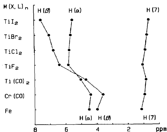
Fig. 1. ^1\text{H} -NMR shifts for \alpha and \beta cyclopentadienyl and tetramethylethano protons in various (\text{CH}_3)_4\text{C}_2(\text{C}_5\text{H}_4)_2\text{M}(\text{X},\text{L})_n complexes.
