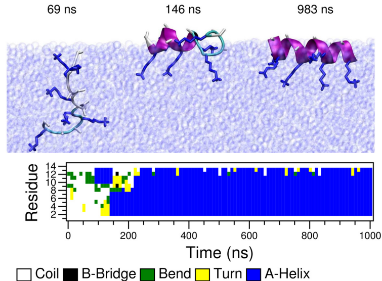
Fig 5. Time evolution of secondary structure of a single AK (in-silico mutated form of LK) peptide at the vacuum/water interface. Initially the peptide is submerged in bulk water and moves to the interface in 80 ns and remains there for the rest of the simulation.
