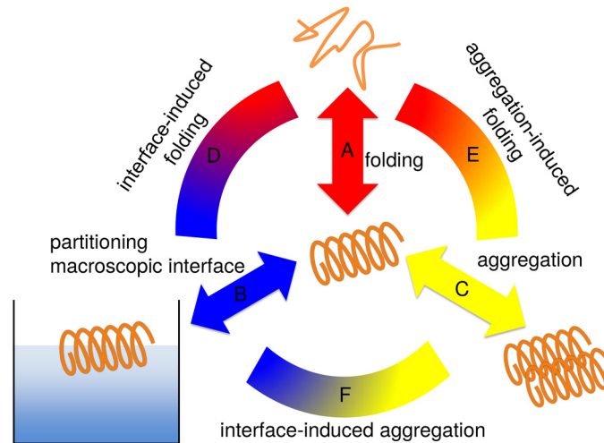
Fig 2. Three separate contributions govern the dynamic conformational equilibrium of an amphiphilic peptide. The folding of the individual molecule in solution (A); the partitioning of hydrophobic/hydrophilic residues induced by macroscopic interfaces (B) or molecular interfaces upon aggregation (C). Combinations of these effects (connecting arcs D, E and F) determine the preferred secondary structure in a given environment.
