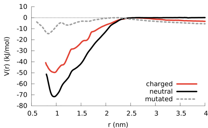
Fig 7. PMF results comparing the separation of a LK dimer in bulk water for the cases where lysine residues are positively charged, lysine residues are neutral and the leucine residues are in silico mutated to alanine residues. The curves are shifted so that the maximum points are zero. The distance refers to the distance between the center of mass of backbone atoms of the peptides. For the mutated AK dimer, when the peptides are in contact they maintain their helical structures. However when they are separated or when they make a loose contact the \alpha -helical structure is not conserved.
