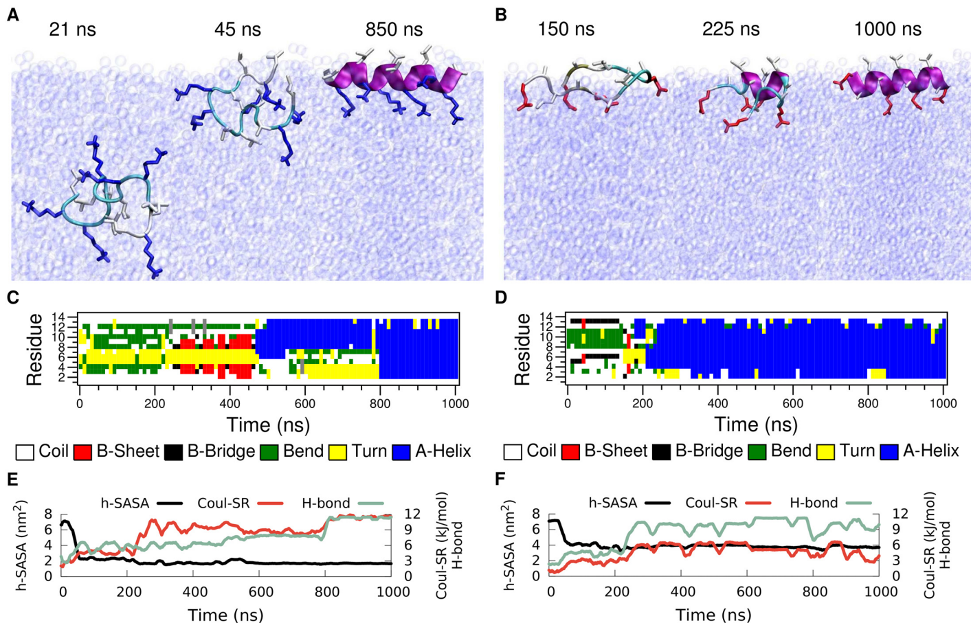
Fig 4. Simulations of a single peptide at the vacuum/water interface for LK (left) and EALA (right). Simulations are started with random conformations at the center of the water slab. Upon adsorption of peptides (after 45 ns for LK and 50 ns for EALA) partitioning of hydrophobic/hydrophilic residues and folding into the \alpha -helix structure (after 800 ns for LK and 350 ns for EALA) is observed. Snapshots depicting the adsorption and adoption of the \alpha -helix structure (A and B) and the DSSP analysis of the secondary structure evolution (C and D) are shown for both molecules. SASA, intra-peptide backbone hydrogen bonds and short-range Coulomb interaction energies between the charge groups (E and F) display the partitioning of hydrophobic/hydrophilic residues and secondary structure formation in the presence of the interface.
