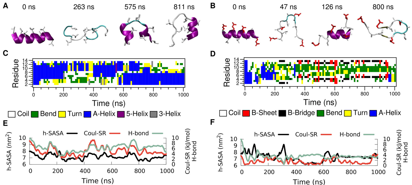
Fig 3. Time evolution of secondary structure for LK (left) and EALA (right) when isolated in bulk water. Snapshots depicting various conformations adopted by these molecules (A and B), DSSP analysis of secondary structure (C and D), SASA for hydrophobic sidechains (h-SASA), number of intra-peptide backbone hydrogen bonds (H-bond) and short-range Coulomb interaction energies (Coul-SR) between the charged groups (E and F) are given for both of the molecules. See Methods section for the color coding and representation of peptides in A and B.
