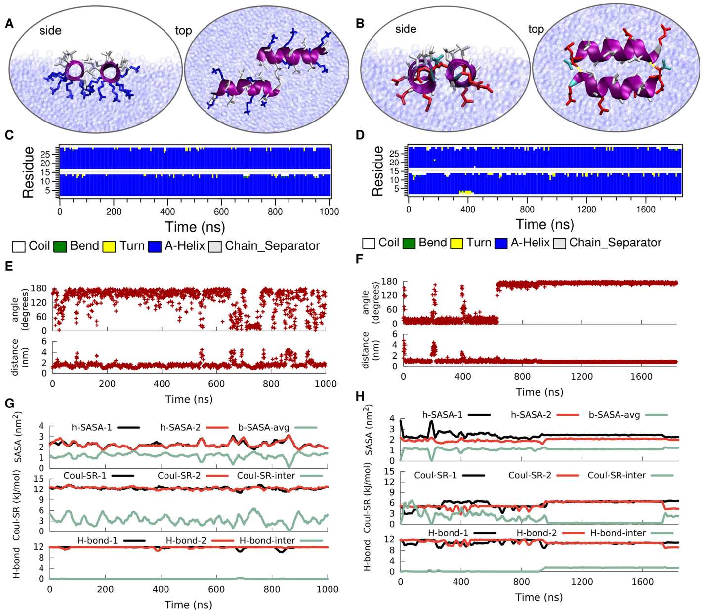
Fig 8. Time evolution of the secondary structure of a dimer of LK (left) and EALA (right) at the vacuum/water interface. Typical snapshots when the peptides are associated at the interface (A and B), DSSP structural analysis (C and D), angle between the helix axis for the peptides and center-to-center distance (E and F), the h-SASA for each peptide along with the buried SASA for the whole peptide, the inter and intra molecular short-range Coulomb energies and the number of inter- and intra-molecular hydrogen bonds (G and H) are shown in figure.
