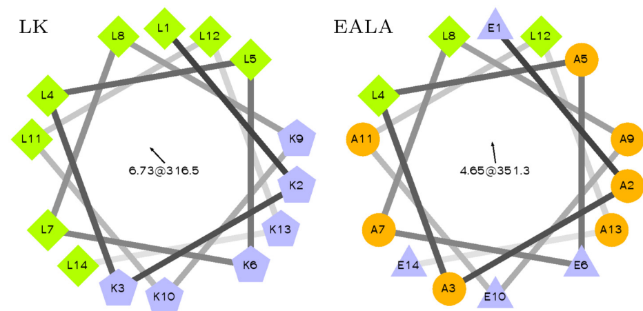
Fig 1. Helical wheel representation of LK and EALA. Both peptides are designed to display secondary amphiphilicity when they adopt the \alpha -helix conformation.
