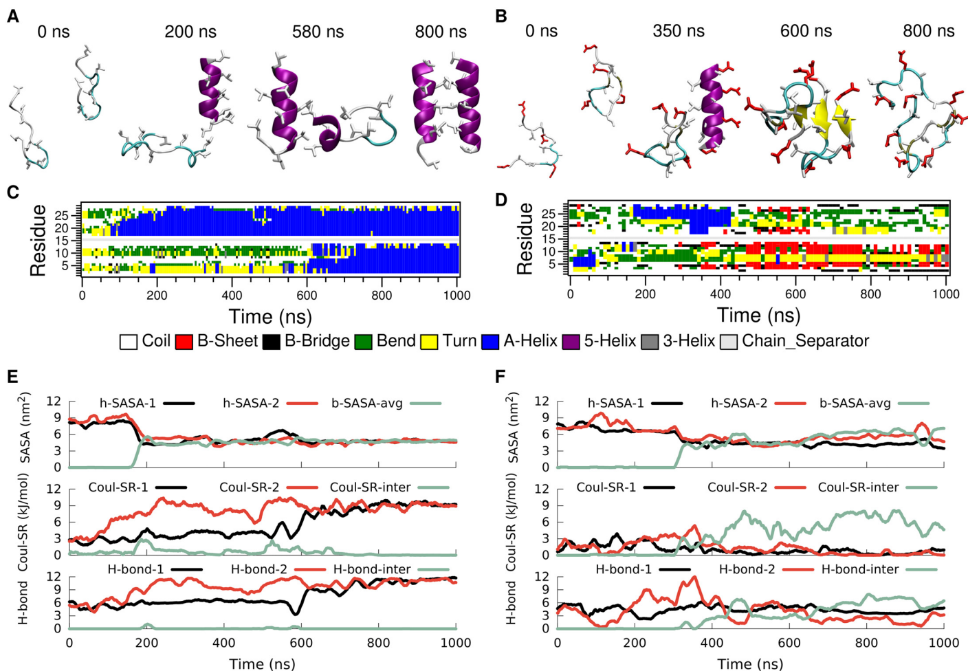
Fig 6. Folding and association of a pair of LK (left) and EALA (right) peptides in bulk water. Snapshots illustrating the aggregation process (A and B), DSSP secondary structure analysis (C and D), SASA, short range Coulombic interaction energies between the charged groups and the number of intra and inter-peptide backbone hydrogen bonds (E and F) are displayed as a function of simulation time. Association of peptides take place at 180 ns for LK and 300 ns for EALA, which can be observed via the sharp drop in SASA.
