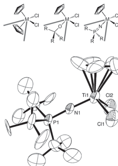
Figure 8. Cone angles of cyclopentadienyl, alkoxy, and phosphinimide ligands [72] and an ORTEP plot of [CpTi(NP t Bu 3 )Cl 2 ]. [76]
