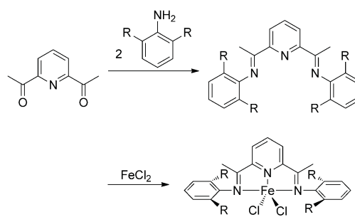
Figure 26. Iron catalyst precursor for linear ethylene polymerization.
