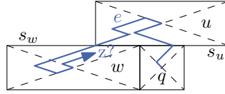
Figure 14: Edges are canonical at one end vertex at least.
