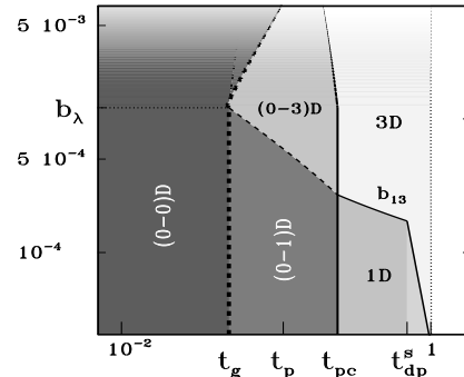
FIG. 2. B - T -pinning diagram of a layered superconductor with decoupled layers (log scales, t = T/T_c , b = B/B_{c2} ; B_\lambda = \Phi_o/\lambda^2 ; parameters for BiSCCO: \lambda = 1800 Å, \xi = 25 Å, d = 15 Å, T_c = 90 K). Results for the various pinning regimes are shown for moderate pinning with T_p = U_p = 10 K. The strong-pinning region at low temperatures T < T_{pc} is divided into two parts: At T < T_g thermal effects are irrelevant [(0-0)D regime], while at T_g < T < T_{pc} variable-range thermal smoothing takes place [(0-1)D and (0-3)D regimes]. The dashed fat line at T = T_g indicates the jump in the collective pinning length L_g and the critical current density j_g . At temperatures T > T_{pc} and low inductions vortex segments of length L_c > \lambda are pinned collectively (1D regime). The remaining area shows the 3D (vortex-bundle) pinning regime.
