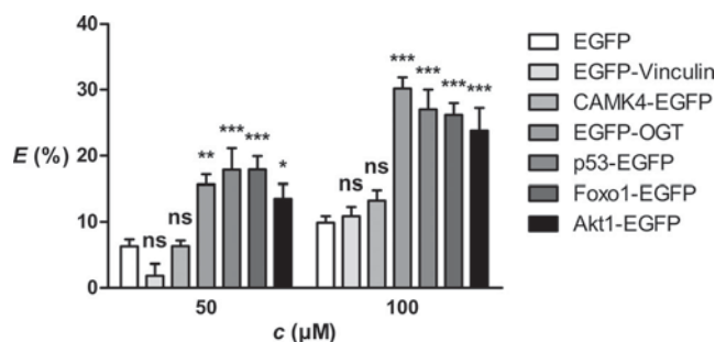
Figure 4. Comparison of the FRET efficiencies of all of the studied proteins. Fluorescence modulation lifetimes from 15 cells from 3 independent experiments, using sugar concentrations ( c ) of 50 μM or 100 μM, were averaged and apparent FRET efficiencies ( E ) were calculated. Mean values ± SEM are depicted. Statistical significance was assessed with a two-way ANOVA and a Bonferroni posttest. The degree of significance is ns = not significant, * p < 0.05, ** p < 0.01, and *** p < 0.001.
