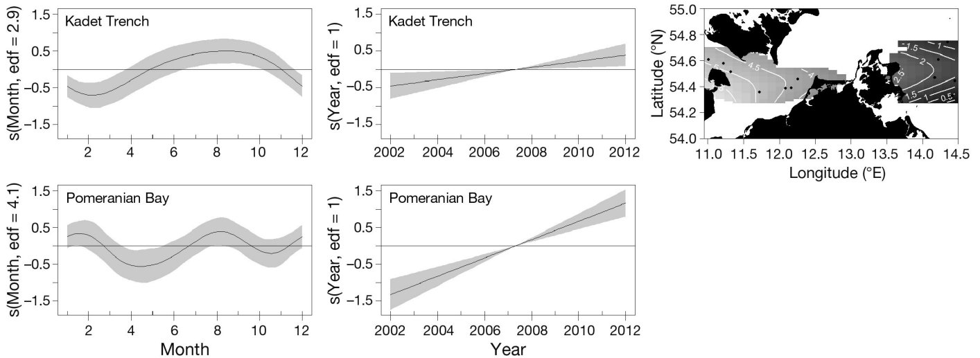
Fig. 5. General Additive Mixed Model (GAMM)-smoothers for significant co-variables when modelling distribution, seasonal patterns and annual differences of the detection positive days per month ( \text{DPD mo}^{-1} ) for the areas Kadet Trench and Pomeranian Bay. Dots in the upper right graph represent the monitoring positions. edf = estimated degrees of freedom; s = smoother. The contour plot shows the log-scaled (link) dependency of \text{DPD mo}^{-1} for the tensor product of Latitude and Longitude with decreasing impact from light to dark colours indicating higher densities in westerly waters
