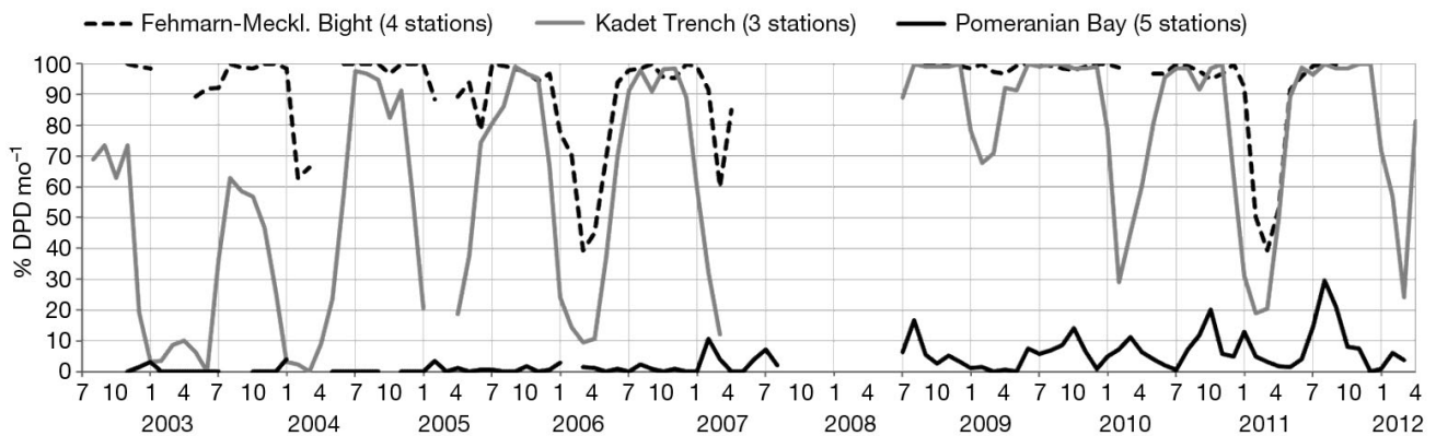
Fig. 4. Proportion of detection-positive days per month (DPD \text{mo}^{-1} ) for the areas Fehmarn/Mecklenburg Bight, Kadet Trench, and Pomeranian Bay from west to east along the German Baltic Sea coast. x-axis: month and year
