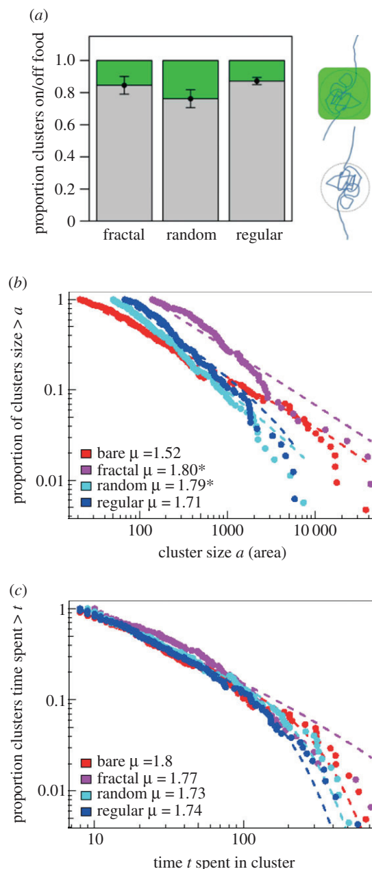
Figure 3. Cluster analysis results in relation to food encounter. (a) Proportion of ARS clusters on bare mud (light grey) and food patches (green; dark grey); see examples of search clusters on the right. Error bars are standard errors of the proportion of clusters on bare mud. (b) Cumulative inter-patch (i.e. off-food) cluster size distributions (tail) grouped by landscape type. Dashed lines indicate the best fit to each dataset; hyperexponential ( k = 3 ) for the bare and regular landscapes, and truncated power-law for the fractal and random landscapes. (c) Cumulative distributions (tail) of time spent in inter-patch ARS clusters grouped by landscape. Dashed lines are best-fit hyperexponentials ( k = 3 ) for all landscapes. Power-law scaling exponents are provided for all distributions; asterisks (only in (b)) indicate distributions for which power-law fits were superior to hyperexponentials. (Online version in colour.)
