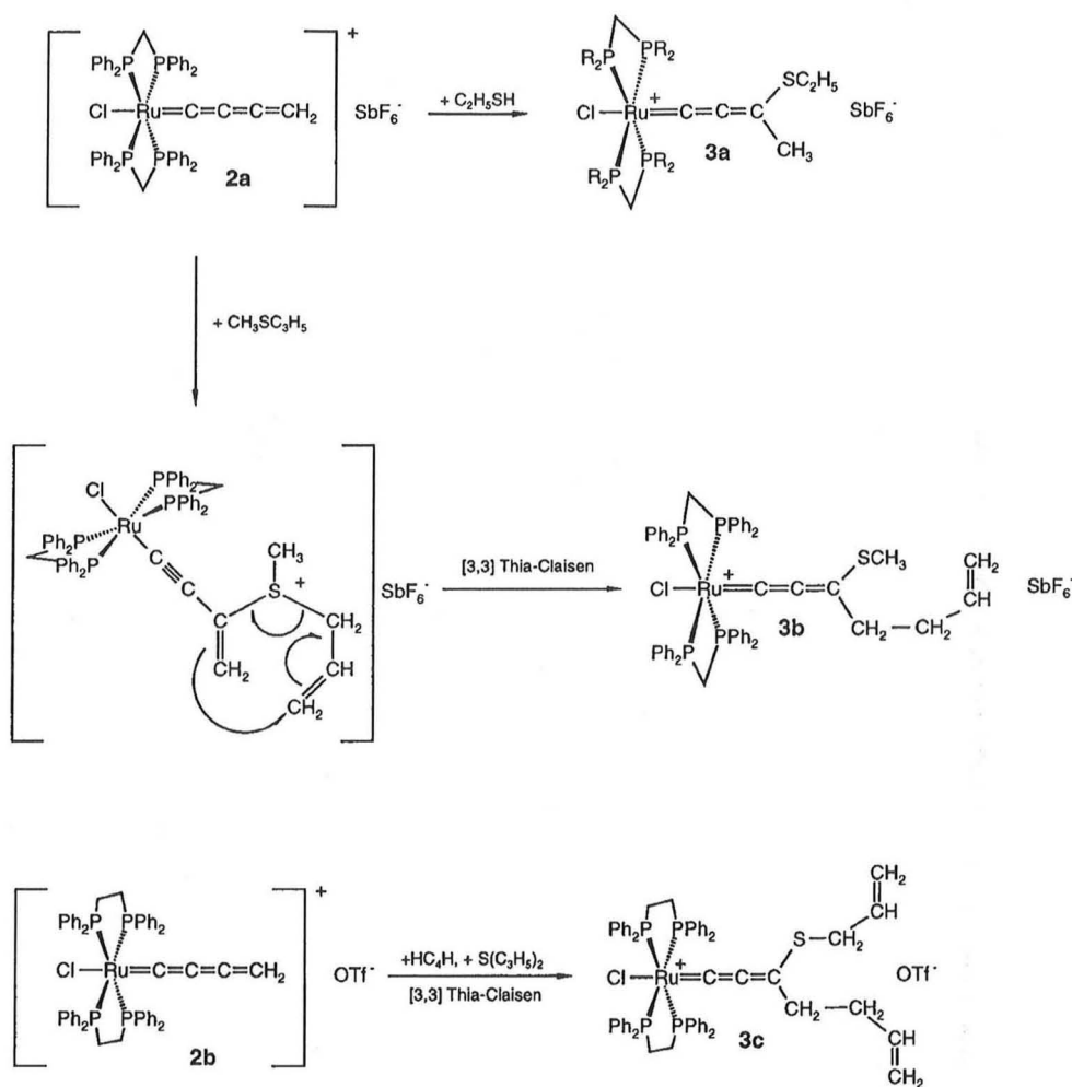
Scheme 1. Synthesis of the thioallenylidene complexes 3a–c
