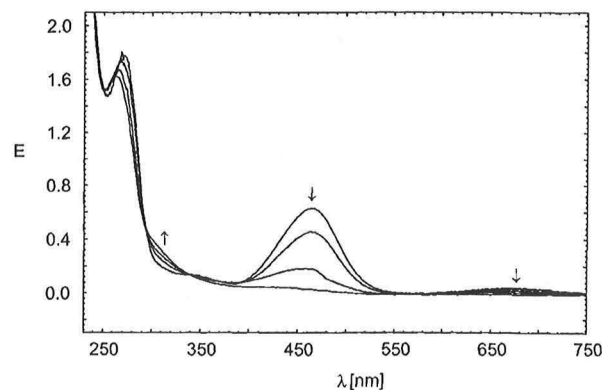
Figure 4. UV/Vis spectroscopic changes during the reduction of trans -[Cl(dppm) 2 Ru–C≡C–C(SMe)C 4 H 7 ] + ( 3b )
