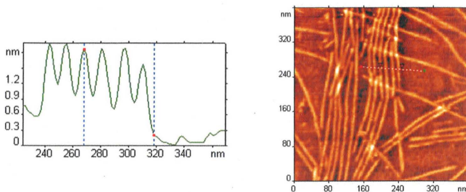
Figure S3. AFM height image and height profile (z range 2 nm, mica) of self-assembled I .
