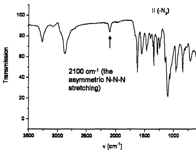
Figure S4. ATR-FT IR of the azide functional conjugate (II).
