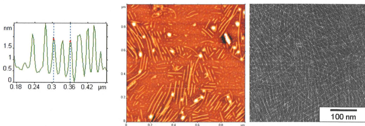
Figure S7. Self-assembled nanotapes of II . AFM height image and height profile (middle and left, z range 3 nm, mica) and TEM micrograph on carbon coated copper grid (right, negative stained with 10 Uranyl acetate).
