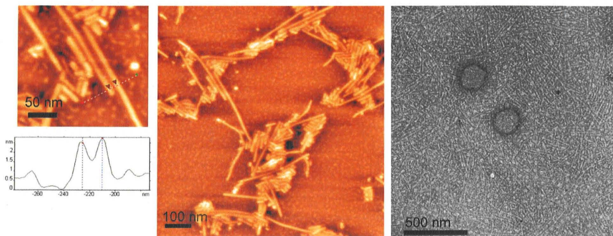
Figure S14. Micrographs of pentinoic acid modified fibres (IV b). AFM height image (middle), the corresponding height profile (left) (z range 3 nm, mica) and a TEM micrograph (right) on carbon coated copper grid (negative stained with uranyl acetate). (AFM: 15.3 nm width, 1.86 nm height; TEM: 16.7 nm width).
