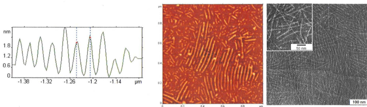
Figure S10. Self-assembled nanotapes of III b . AFM height image (middle) and corresponding height profile (left) (z range 3 nm, mica) and TEM micrograph (right) on carbon coated copper grid (negative stained with Uranyl acetate).
