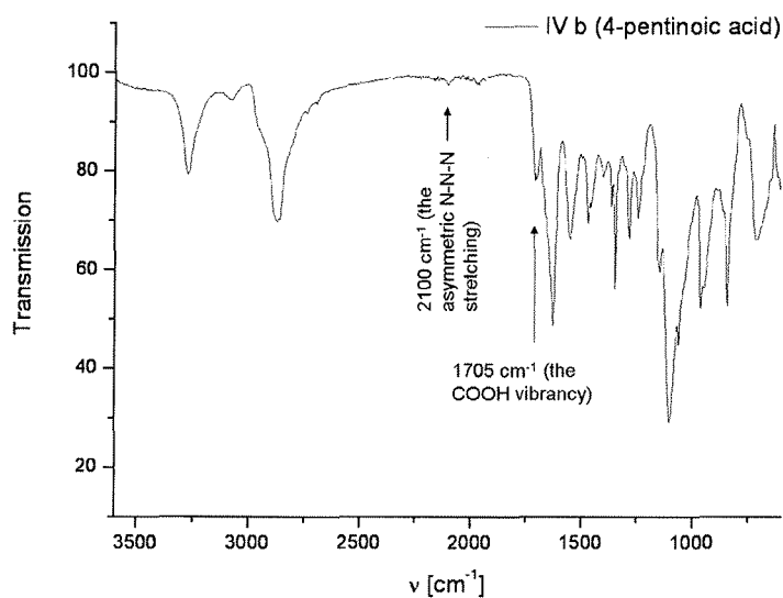
10 Figure S12. ATR-FT IR of the pentinoic acid functional conjugate (IV b).
