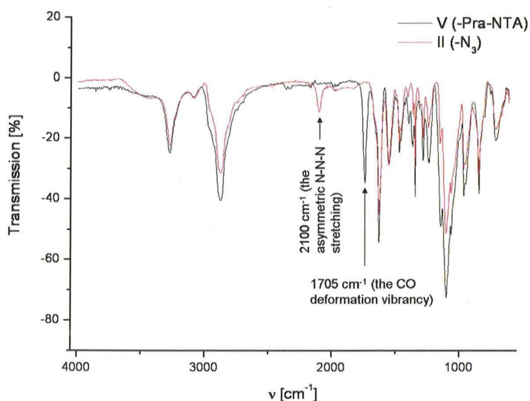
Figure S15. ATR-FT IR of the Pra-NTA functional conjugate (V b).
