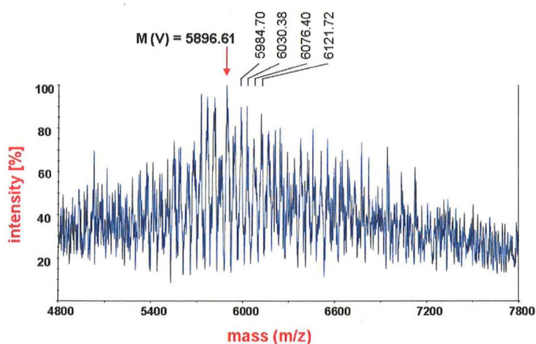
Figure S17. MALDI-TOF-MS of V b (DHB as matrix).
