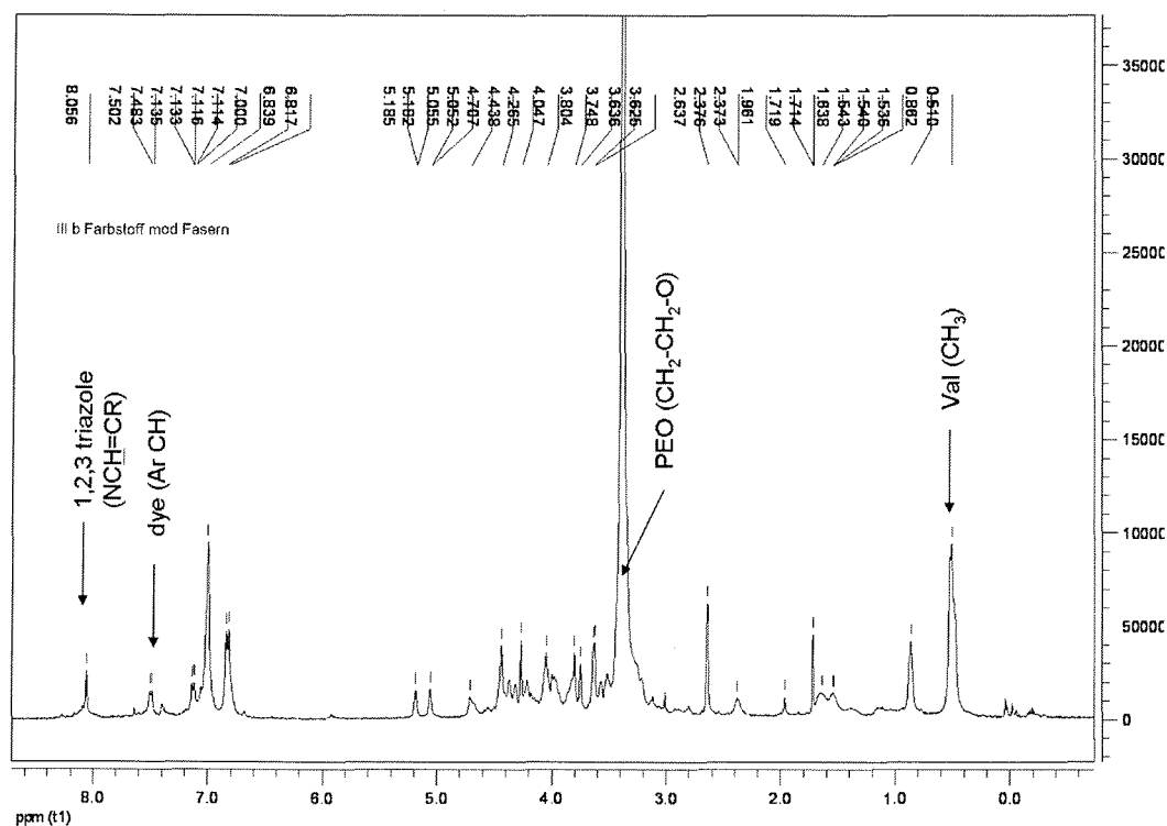
Figure S9. 1 H-NMR of the dye functional conjugate in TFA ( III b ).
