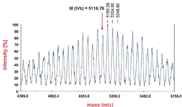
Figure S13. MALDI-TOF-MS of IV b (ACHC as matrix).
