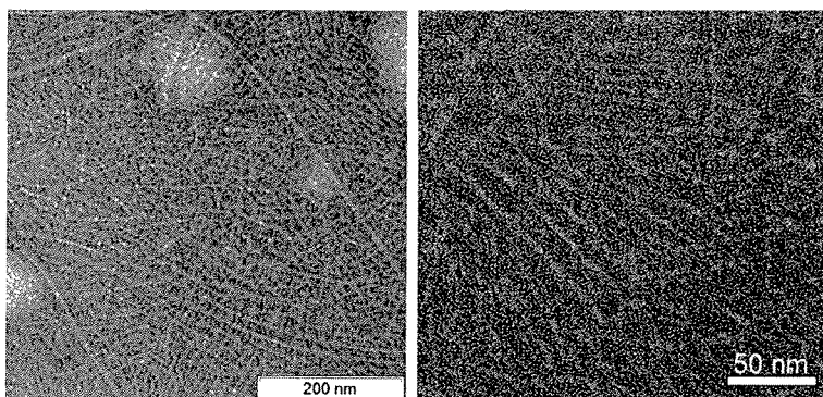
Figure S18. TEM micrographs of Pra-NTA modified fibres (V b; Evaluation: 17.0 nm width, 3.88 nm unstained core).
