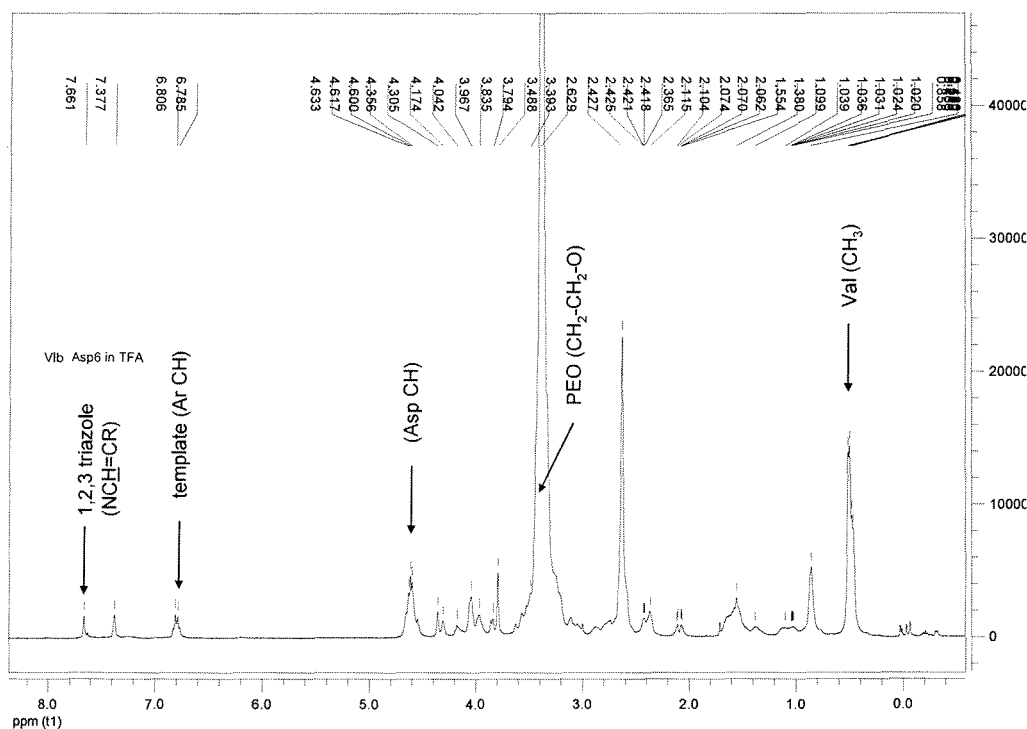
Figure S20. 1 H-NMR of the Asp 6 functional conjugate (VI b).
