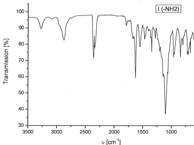
Figure S1. ATR-FT IR of the amine functional conjugate ( I ).
