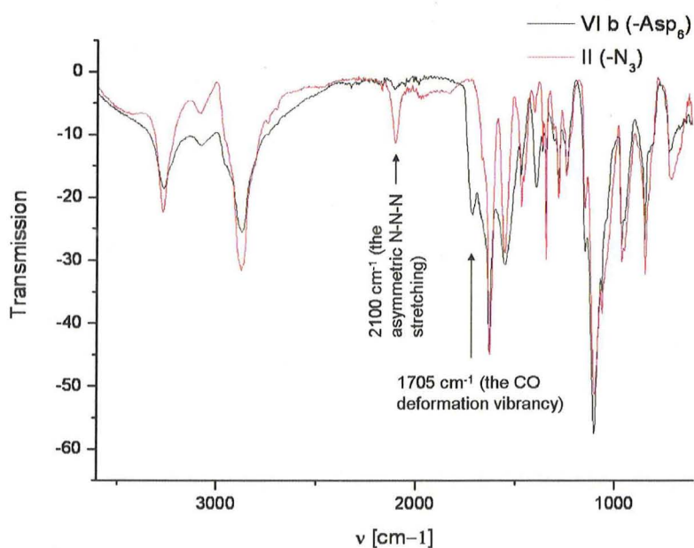
Figure S19. ATR-FT IR of the Asp 6 functional conjugate (VI b).
