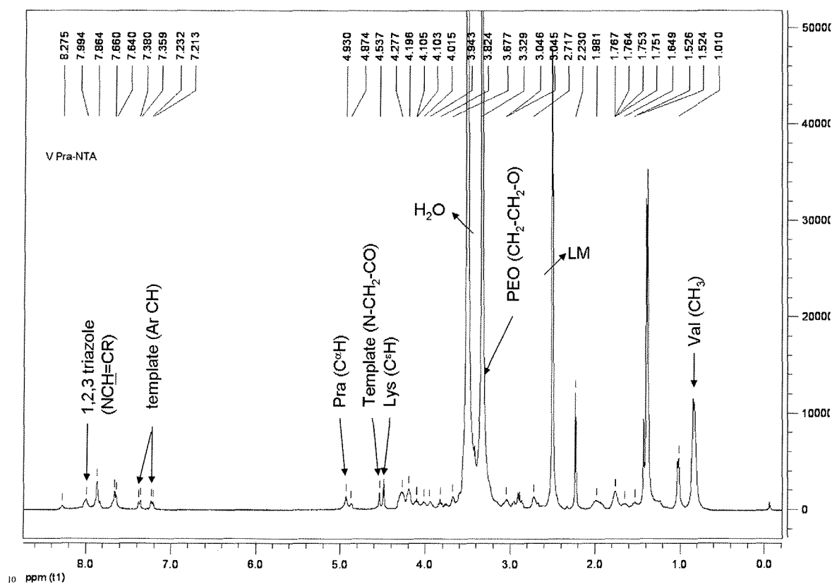
Figure S16. 1 H-NMR of the Pra-NTA in DMSO functional conjugate (V b).
