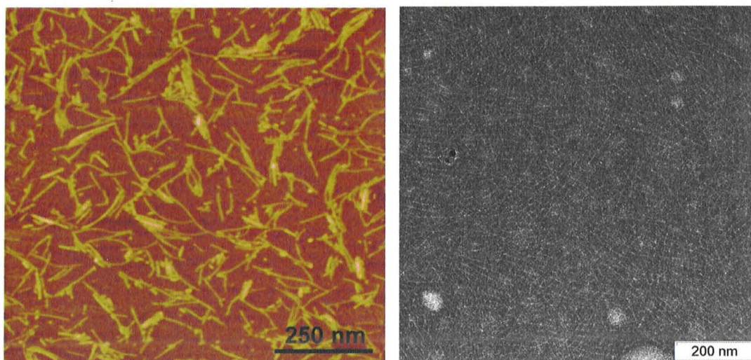
Figure S21. Micrographs of asparagine acid hexapeptide modified fibres ( VI b ). AFM height image (left 10 z range 3 nm, mica) and TEM micrograph (right) on a carbon coated copper grid (negative stained with Uranyl acetate). (Evaluation: AFM: 1.8 nm height; TEM 15 nm width).
