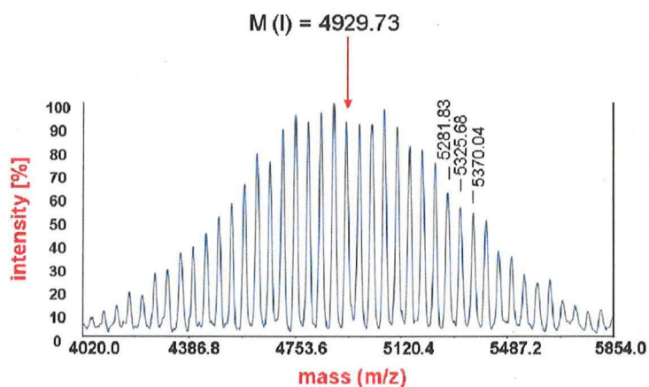
Figure S2. MALDI-TOF-MS of the amine functional conjugate ( I ).
