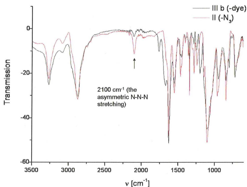
Figure S8. ATR-FT IR of the dye functional conjugate ( III b ).
