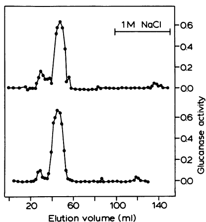
FIG. 3. CM-cellulose chromatography on Whatman CM52 of peak a from chromatofocusing (top) and peak f (bottom). The column (2.2 × 16 cm) was equilibrated and eluted with 50 mM Na-citrate (pH 5.5). Fractions (2.1 mL) were collected at a flow rate of 6.3 mL/h. Washing with 1 M NaCl in elution buffer did not elute more activity. (●—●) β-1,3-glucanase activity.
