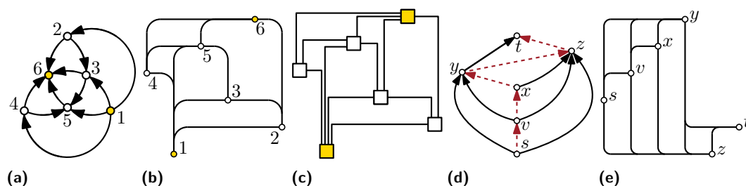
■ Figure 1 (a) A bitonic st-orientation that admits an upward-planar L-drawing (b). (c) The corresponding drawing in the Kandinsky model. (d) An upward-planar st-graph that does not admit an upward-planar L-drawing. (e) A planar L-drawing of the graph in (d).
