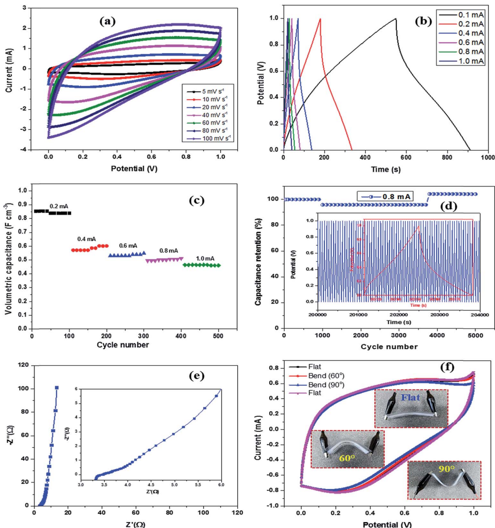
Fig. 4 Electrochemical evaluation of the 3D-NCO/Ni//3D-NCO/Ni solid state symmetric device. (a) Cyclic voltammograms of the solid state symmetric device as a function of scan rate. (b) Galvanostatic charge/discharge voltage profiles at different currents. (c) Cycling performance of the 3D-NCO/Ni//3D-NCO/Ni symmetric fiber supercapacitor with increasing currents. (d) Cycling performance of the fiber supercapacitor measured at a constant current of 0.8 mA; the inset displays the charge/discharge curves at 0.8 mA. (e) Nyquist plot of the symmetric device; the inset shows the magnified plot in the high-frequency region. (f) CV curves of the fiber supercapacitor at different bending states; the inset shows the digital camera images of the device at different bending states.
