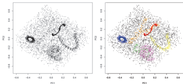
Fig. 3. PCA projection of data displayed in Figure 2. The dataset contains six clusters (highlighted on the right). Two clusters are hardly recognizable in the PCA projection (orange Y and green S).
