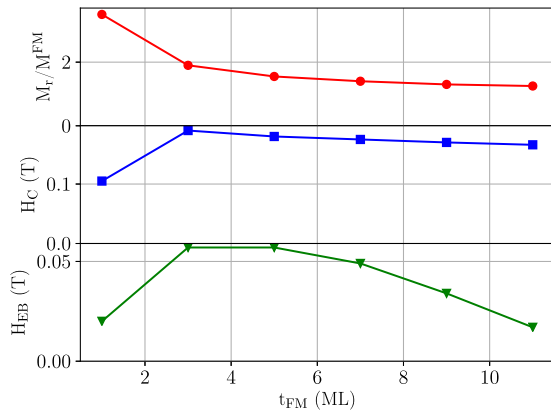
FIG. 11. Calculated relative remanence magnetization, coercive, H_C , and exchange-bias fields, H_{EB} , as a function of the FM thickness, t_{FM} , in the case of t_{AF} = 25 ML.
