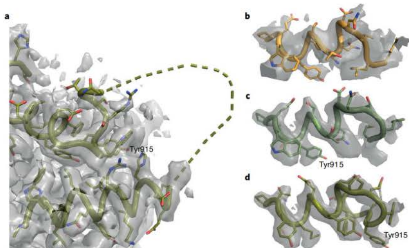
Fig. 2 | Register shift in the C terminus of RNA polymerase. a , Overview with missing loop shown as a dashed line (PDB 7BV2); map at 2.4\sigma . Right, details of the C-terminal helix at 5\sigma . b , Lower resolution map and model (PDB 6NUS). Judging the side chain fit is difficult. c , Higher resolution map and model (PDB 7BV2) as deposited; the side chain fit is suboptimal due to the register error. d , Amended model for PDB 7BV2; the side chains now fit the density. The register shift is indicated by the labelled Tyr915. Picture: CSTF/insidecorona.net.
