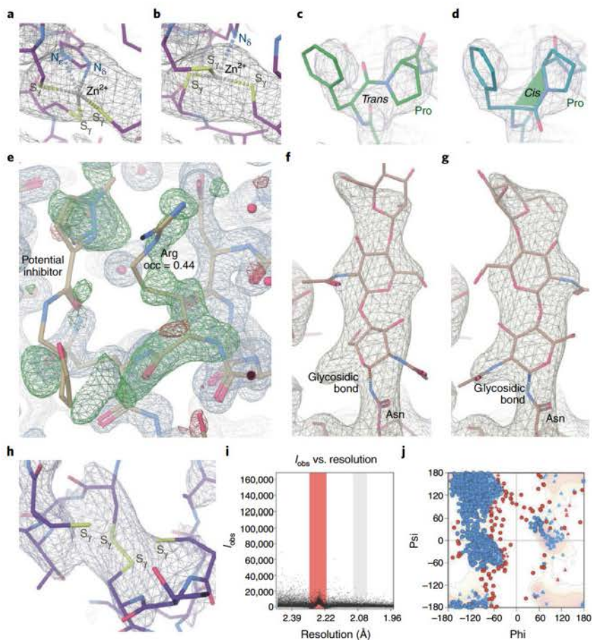
Fig. 1 | Examples of common errors and improvements. All pictures except i are screenshots from the Coot v0.9.9 prerelease. Residual density and reconstruction maps are in blue-gray, difference electron density in red and green. a , SARS-CoV-1 Nsp14-Nsp10 (PDB 5CBT) histidine zinc-coordination site (B603), with residual density contour level 0.445, root mean square deviation (r.m.s.d.) 0.150. b , Histidine from a has been swapped in ISOLDE 25 , leading to tetrahedral coordination of Zn 2+ , then refinement was performed using PDB-REDO 11 with manual addition of links. c , Proline A505 is modelled as trans in the RdRp complex (PDB 7BV2, left), but the density indicates a cis main chain conformation, shown in d . e , High difference electron density at residue A165 in the SARS-CoV-2 main protease (PDB 5RFA) due to an occupancy of only 0.44 rather than 1.00 near the potential inhibitor (left). Residual map contour level 0.54, r.m.s.d. 0.319; difference density at contour level 0.35, r.m.s.d. 0.114. f , SARS-CoV-2 spike receptor-binding domain complexed with human ACE2 (PDB 6VV1). This N-linked glycan is flipped approximately 180° around the N-glycosidic bond. After we contacted the original authors, this entry was revised (shown in g ). g , Correction improves the density fit of the sugar chain. Residual map at contour level 0.311, r.m.s.d. 0.265. h , Disulfide bond A226-A189 in papain-like protease (PDB 6W9C), with electron density at contour level 0.214, r.m.s.d. 0.136; the other two cysteine residues remain uncoordinated. While the density map does not indicate a zinc, it is a zinc finger domain; the other NCS copies include a coordinated zinc at this position. i , AUSPEX 8 plot of SARS-CoV main protease (PDB 2HOB); ice rings are reflected by a bias in the intensity distribution (red). j , Ramachandran plot or torsion angles in the peptide backbone for the SARS-CoV Nsp10-Nsp14 dynamic complex (PDB 5NFY). In principle, there should only be a few outliers (red), as most peptide bonds adhere to typical angular distributions. Picture: CSTF/insidecorona.net.
