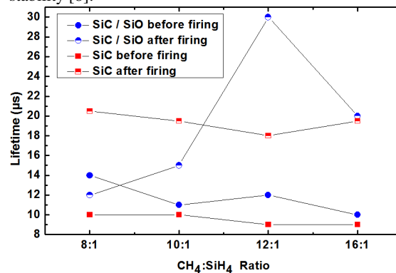
Figure 3: Minority charge carrier lifetimes (measured by QSSPC) of mc wafers with different surface passivation layers before and after a firing step (peak temperatures \sim 860 \text{ }^\circ\text{C} ).
