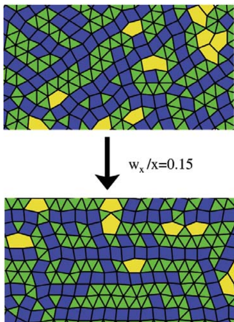
Fig. 13. Stabilization by a phasonic gradient: Archimedean-like tiling phase (same parameters as in fig. 10) obtained by Monte Carlo simulations without phasonic displacement (top) and in a potential with a phasonic gradient with w_x/x = 0.15 (bottom).
