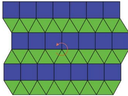
Fig. 4. (Colour on-line) Archimedean tiling of type (3^3 \cdot 4^2) .
