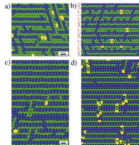
Fig. 1. Archimedean-like tiling phases induced by (a,b) decagonal and (c,d) tetradecagonal substrates. (a,c) show experimental results, (b,d) are obtained by Monte Carlo simulations. The figures show Delaunay triangulations of colloidal point patterns. Bonds longer than 1.1a_S ( 1.2a_S for experiments) are omitted, where a_S is the spacing of the particles when placed on an ideal triangular lattice. The potential strength is V_0/(k_B T) = 13 in (a), V_0/(k_B T) = 10 in (c), and V_0/(k_B T) = 20 in the simulations (b,d). The density is given by a_S/a_V = 0.57 in (a), a_S/a_V = 0.58 in (b), and a_S/a_V = 0.7 in (c,d).
