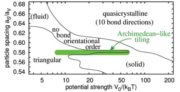
Fig. 3. (Colour on-line) Phase diagram obtained with Monte Carlo simulations for colloids on the decagonal substrate (the complete phase diagrams are presented and explained in [19]). Unlike quasicrystalline phases that we observed at all densities, Archimedean-like tiling structures are only found for intermediate potential strengths within a small range of densities (marked green).
