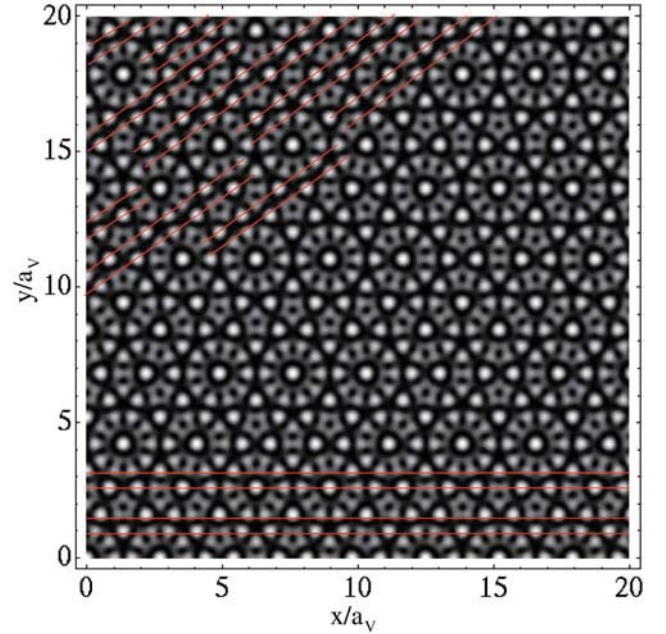
Fig. 12. (Colour on-line) Interference pattern of the decagonal laser field calculated from eq. (1) when the phase \phi_0 attached to the wave vector \mathbf{G}_0 varies with a constant gradient, \phi_0 = 0.2x/a_V . Via eq. (2) one can show that it creates a constant gradient in the x components of the phasonic and phasonic displacements. As a result, the lines of low intensity are infinitely extended in the x -direction whereas in all other directions they have a finite length (see, e.g. , the dark stripes framed by the red lines). Similar jags are studied in [24,25].
