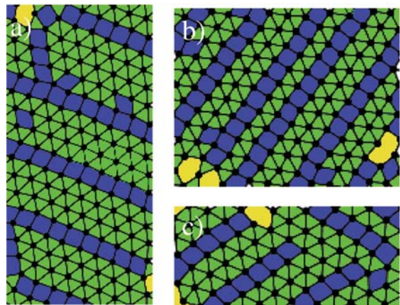
Fig. 14. Delaunay construction (as in fig. 1) of simulation results that consist of rows of triangles and rows of squares in laser fields (of strength V_0/(k_B T) = 50 ) created by (a) eight beams ( a_S/a_V = 0.8 ), (b) ten beams ( a_S/a_V = 0.7 ), and (c) eleven beams ( a_S/a_V = 0.74 ).
