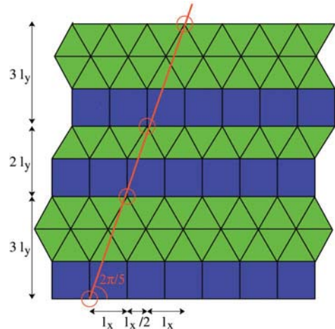
Fig. 6. (Colour on-line) We calculate the mean bond length in horizontal direction l_x in a way that many colloids lie along the 2\pi/5 -direction (circled in red). The mean row height l_y is chosen to fit one of the two length scales of the substrate in the y -direction.
