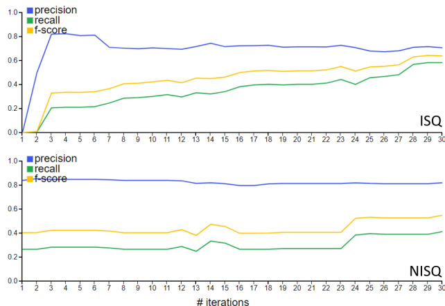
Figure 6: Performance of Setting 1 for 30 learning iterations: Precision stays stable for both question types while recall steadily increases for ISQ.
