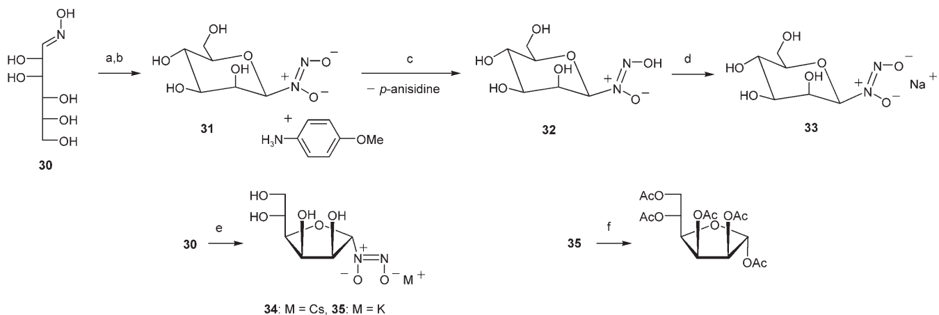
Scheme 4. Reactions of mannose oxime with NO^+ . a) NaNO_2/HCl . b) p -Anisidine. c) THF/MeOH. d) NaHCO_3 . e) Me_2CHCH_2CH_2-ONO , H_2O , M^+ OH^- . f) Ac_2O /pyridine, 5 °C.
