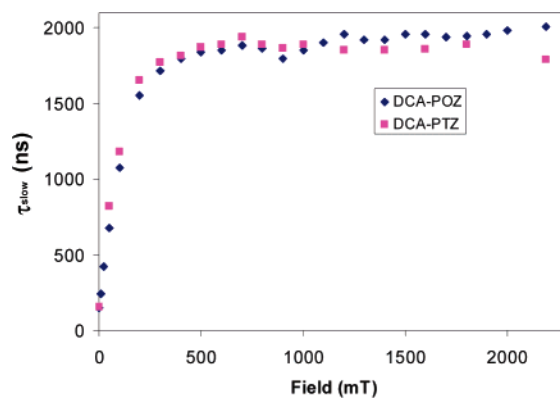
Figure 5. \tau_{\text{slow}} vs B for DCA-PTZ and DCA-POZ.
