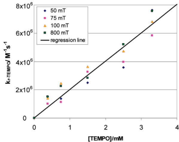
Figure 11. Contribution k_{r,TEMPO} to spin relaxation as a function of TEMPO concentration for various magnetic fields.
