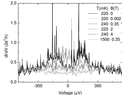
FIG. 6: Differential conductance, calculated numerically from the IVs of Fig. 5. For clarity, the reproducibility is only shown for the curves recorded at B = 0 and B = 2 T.
