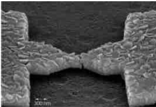
FIG. 1: Electron micrograph of sample No. 1 under an inclination angle of 70^\circ , taken after measurement. The polycrystalline structure of the Zn film is clearly visible. A remaining spacing of the bridge arms of several nm and a fine nanowire between them is observed.
