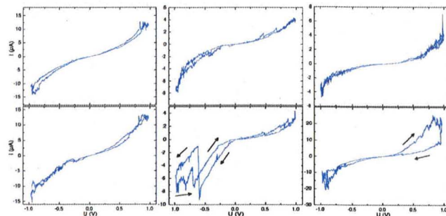
Fig. 5. Selection of I - V curves measured on BTT.
