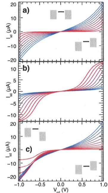
Fig. 3. I - V curves calculated for different values of \Gamma and E_0 in the single level model. (a) Variation of \Gamma in a symmetric junction. The position of the molecular level was fixed at E_0 = 0.5 eV, 0.01 eV \leq \Gamma \leq 0.1 eV. (b) Variation of E_0 in a symmetric junction. \Gamma = 0.03 eV, 0.3 eV \leq E_0 \leq 0.7 eV. (c) Variation of \Gamma_1 in an asymmetric junction. \Gamma_2 = 0.1 eV, E_0 = 0.5 , 0.01 eV \leq \Gamma_1 \leq 0.1 eV.
