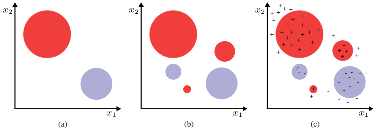
Figure 2: Shows a two-level rule hierarchy. (a) Two top-level rules assigned to two different classes, + (red) and - (blue), (b) three additional rules on the next level, (c) all rules together with their underlying data points.
