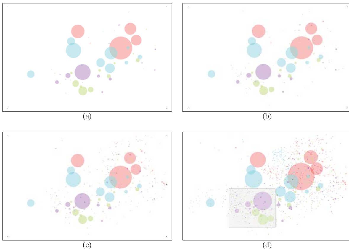
Figure 5: Stepwise rule hierarchy projection on vehicle data starting from top- to bottom-level (a)-(c), and (d) rules of all levels and data points.
