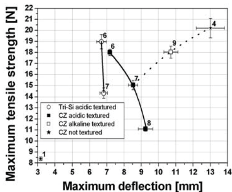
Figure 5: Mean values of the maximum breakage forces over the maximum displacement for different surface morphologies. The solid lines are only guides to the eye.
