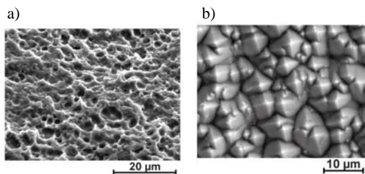
Figure 3: Scanning electron microscope picture of a) acidic b) alkaline textured CZ wafer surfaces.
