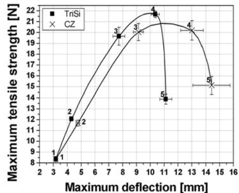
Figure 4: Mean values of the maximum tensile strength in dependency on the maximum displacement of each group. The solid lines are only guides to the eye without experimental background.
