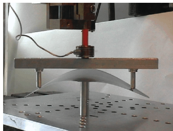
Figure 2: Picture of a CZ wafer right before breaking.
