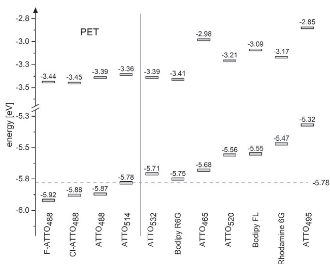
Figure 5. Measured ionisation potentials for eleven different carboxylic acid fluorescence dyes. The LUMO potentials are calculated by adding the absorption maximum. The dashed line corresponds to the HOMO of ATP.
