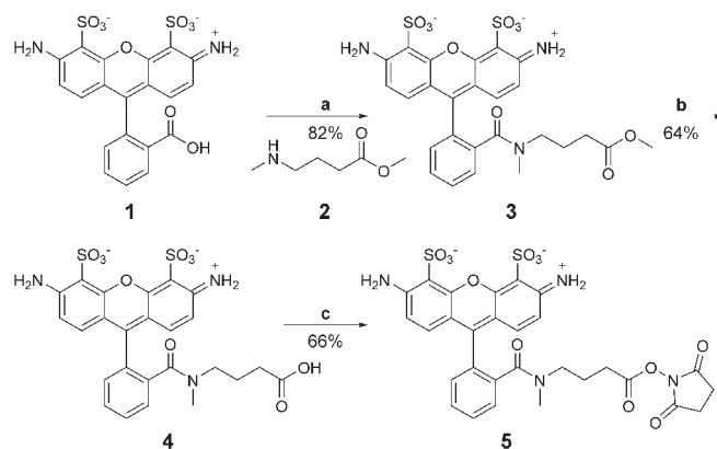
Scheme 1. Synthesis of ATTO 488 NHS: a) methyl 4 (N-methylamino) butyrate, HATU, DMF, Et 3 N, 0 °C, 3 h, b) 2.5 equiv LiOH, 4 °C, 48 h, c) TSTU, Et 3 N, DMF, RT, 2.5 h.
