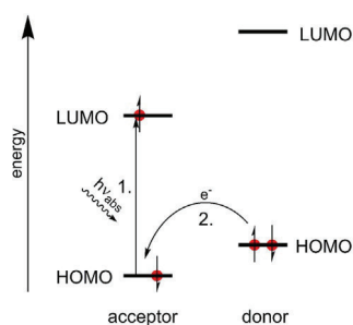
Figure 4. The efficiency of PET is governed by the relative energies of donor and acceptor orbitals.
