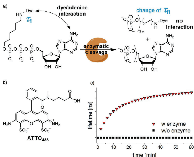
Figure 1. a) General scheme of dye linked ATP: fluorescence lifetime of the attached fluorophore changes when it is in close proximity to the nucleobase. b) Structure of the rhodamine dye ATTO 488 COOH. c) Proposed change of \tau_{fl} when modified ATP analogues are quenched by the nucleobase before cleavage.
