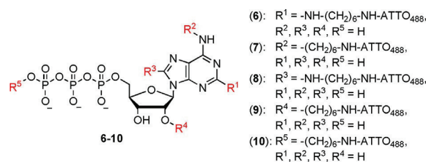
Figure 2. Five synthesised ATTO 488 labelled ATP analogues.
