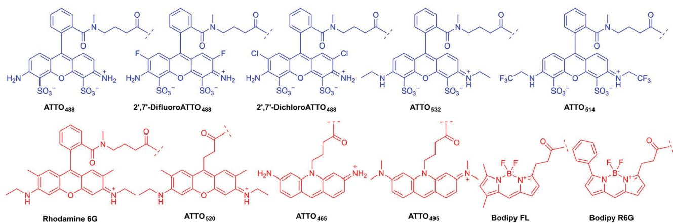
Figure 3. Hydrophilic ATTO 488 core structure (top blue) and hydrophobic (bottom red) fluorescence dyes.
