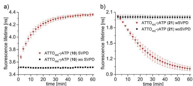
Figure 6. Fluorescence lifetime time course of a) \gamma O (ATTO 488 amidohehyl) adenosine triphosphate and b) \gamma O (ATTO 495 amidohehyl) adenosine triphosphate treated with and without SVPD at 25 °C. All data represent mean \pm standard error of triplicates.
