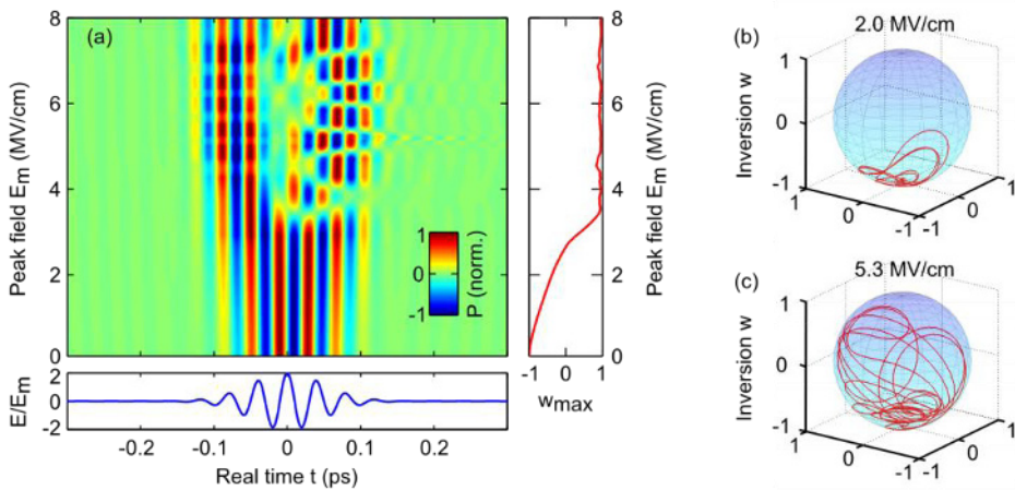
Fig. 2. (a) Normalized polarization response of the two-level system as a function of the real time t and the peak electric field E_m for \tau = 0 ps. Right hand side: Maximum inversion w_{\max} as a function of E_m . Bottom: Driving field of the THz transient. (b,c) Corresponding pathways of the Bloch vector for a moderate ( E_m = 2 MV/cm) and a high ( E_m = 5.3 MV/cm) peak electric field.
