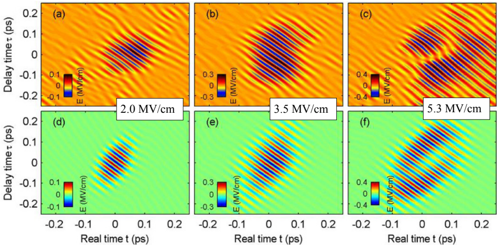
Fig. 1. (a-c) Two-dimensional FWM signatures with external peak fields of the driving transient of 2 MV/cm, 3.5 MV/cm and 5.3 MV/cm, respectively. (d-f) Simulated FWM data reproducing the essential features of the corresponding measured signals above.
