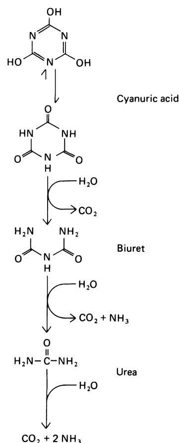
Fig. 3. Degradative pathway of cyanuric acid in Pseudomonas strain D
