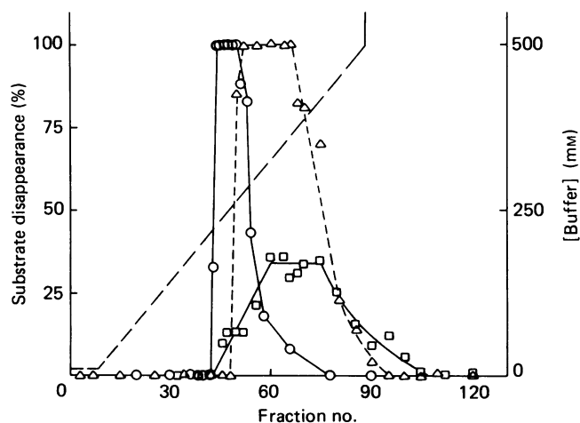
Fig. 2. Separation on DEAE-cellulose of three enzymes of cyanuric acid degradation from strain D
