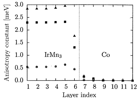
FIG. 4. (Color online) Calculated effective anisotropy parameters (triangles) K_{\text{eff}}^p , see Eq. (32), for the IrMn 3 /Co interface. Also shown are the corresponding one-site ( K_{\text{eff}}^{p,\text{os}} , circles) and two-site ( K_{\text{eff}}^{p,\text{ts}} , squares) contributions.
