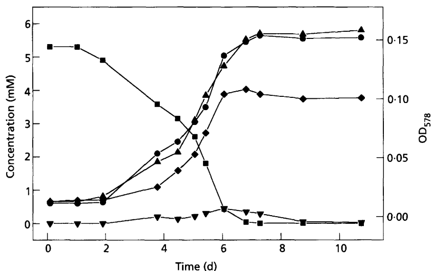
Fig. 2. Growth of strain BT with 5 mM 3-hydroxybenzoate as substrate: cell density (◆), 3-hydroxybenzoate (■), acetate (●), butyrate (▲) and benzoate (▼).
