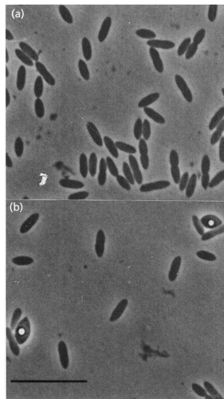
Fig. 1. Phase-contrast photomicrographs of vegetative cells of strain BT (a), and endospore formation in ageing cells (b). Bar, 10 \mu\text{m} .
