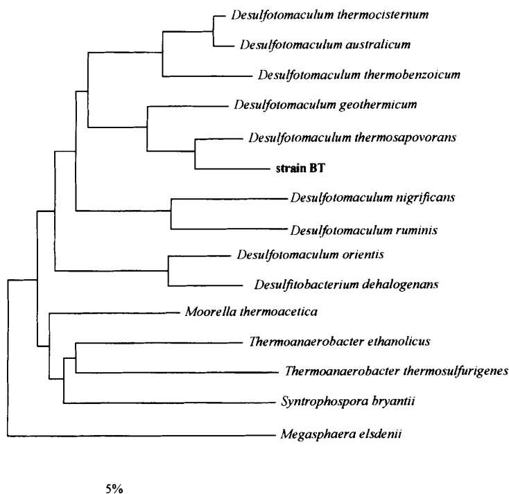
Fig. 3. Phylogenetic dendrogram indicating the position of strain BT within the radiation of the representatives of the genus Desulfotomaculum and related taxa. The scale bar represents 5 nucleotide substitutions per 100 nucleotides.
