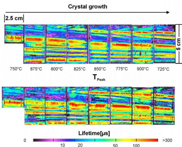
Figure 8: \mu PCD-measurements from adjacent wafers with SiN x fired at different temperatures before (upper half) and after (lower half) an additional MIRHP passivation step.
