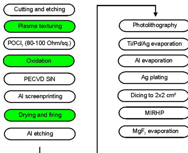
Figure 1: Photolithography based cell process at UKN. Investigated process steps for front side and bulk improvement are highlighted in green.
