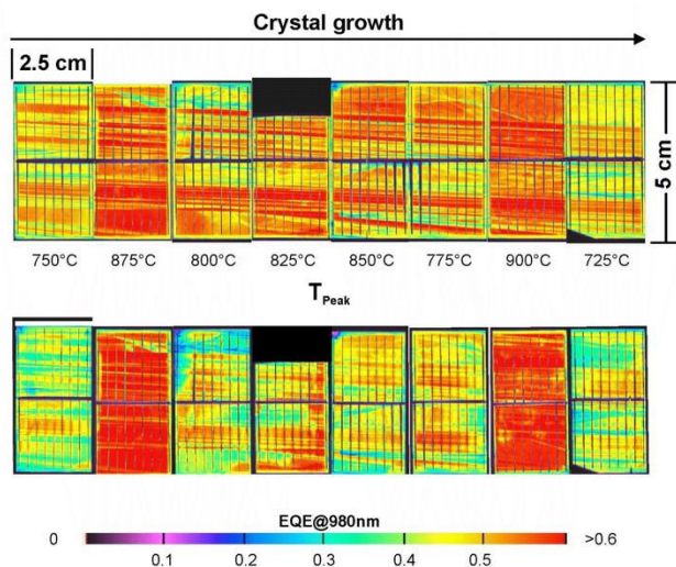
Figure 7: LBIC-results from adjacent cells with SiN x fired at different temperatures before (upper half) and after (lower half) an additional MIRHP-passivation step.
