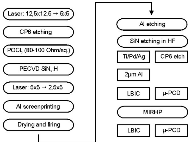
Figure 6: Process for the simplified fabrication of solar cells and lifetime samples. The split up in processing and characterization is shown in the right column (squared fields).
