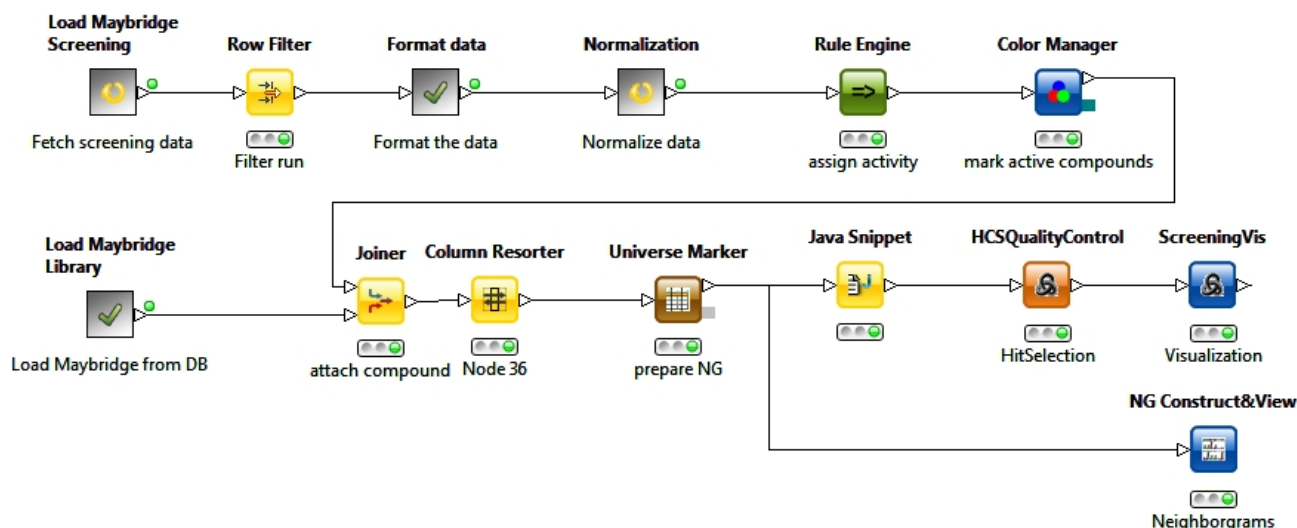
Figure 1. KNIME workflow for high-throughput screening data analysis. The pipeline comprises nodes for data preprocessing (e.g. normalization), interactive plate visualization and for computing neighborgrams.
