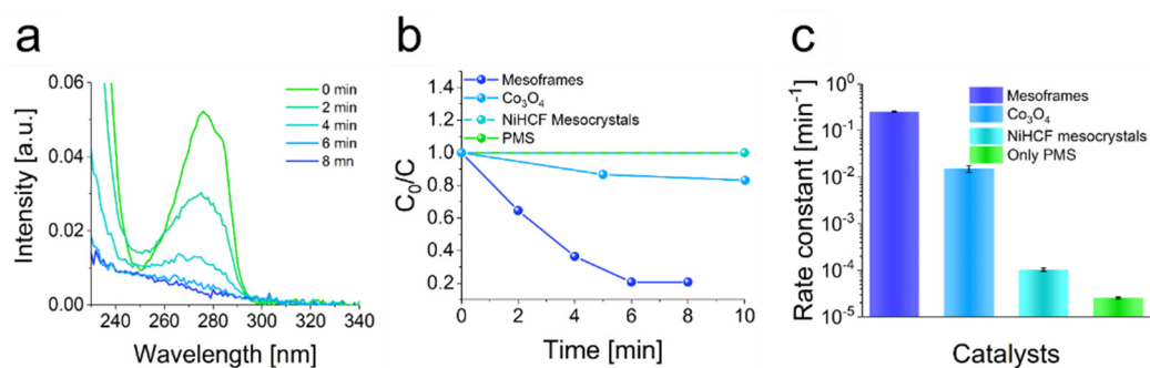
Figure 5. PMS-mediated degradation of bisphenol-A using mesoframes as catalyst. (a) UV-Vis absorption spectra of time-dependent bisphenol-A degradation. (b) Degradation efficiencies of bisphenol-A in the presence of the mesoframes, \text{Co}_3\text{O}_4 , NiHCF mesocrystals and in the absence of any catalyst. (c) Rate constants that correspond to the respective bisphenol-A removals (logarithmic scale for the illustration of all rate constants). Reaction conditions: [\text{Bisphenol-A}] = 40.0 \text{ mg L}^{-1} , V = 100 \text{ mL} , T = 25 \text{ }^\circ\text{C} , \text{pH} = 7 , [\text{Mesoframe}] = 0.20 \text{ g L}^{-1} , [\text{PMS}] = 0.20 \text{ g L}^{-1} .
