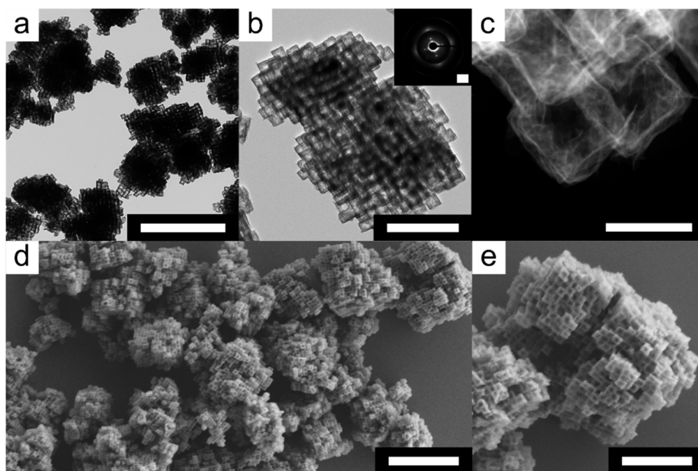
Figure 2. Morphological characterization of the hollow frameworks after alkaline etching. (a) Low and (b) high magnification TEM micrographs of NiHCF mesocrystal-derived hollow frameworks and the corresponding SAED pattern (inset; from the [200] zone axis) obtained from TMAH-mediated etching at room temperature in aqueous media. (c) Dark-field HRTEM micrograph of the NCs on the surface of a hollow framework. (d) SEM micrograph of hollow frameworks distributed on a silicon (100) wafer. (e) High magnification SEM micrograph of a hollow framework. Scale bars: 2.0 \mu\text{m} (top left), 0.5 \mu\text{m} (top middle), 5.0 \text{nm}^{-1} (inset); 100 nm (top right), 2.0 \mu\text{m} (bottom left) and 1.0 \mu\text{m} (bottom right).
