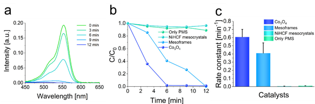
Figure 4. Degradation of rhodamine-B by using mesoframes for PMS-activation. (a) UV-Vis absorption spectra of rhodamine-B degradation within 12 min. (b) Degradation efficiencies of using \text{Co}_3\text{O}_4 , mesoframes and NiHCF mesocrystals as catalysts. The efficiency in the absence of any catalyst is also illustrated. (c) Rate constants derived from the respective degradation curves. Reaction conditions: [\text{Rhodamine-B}] = 10.0\text{ mg L}^{-1} , V = 100\text{ mL} , T = 25\text{ }^\circ\text{C} , \text{pH} = 5 , [\text{Mesoframe}] = 0.10\text{ g L}^{-1} , [\text{PMS}] = 0.30\text{ g L}^{-1} .
