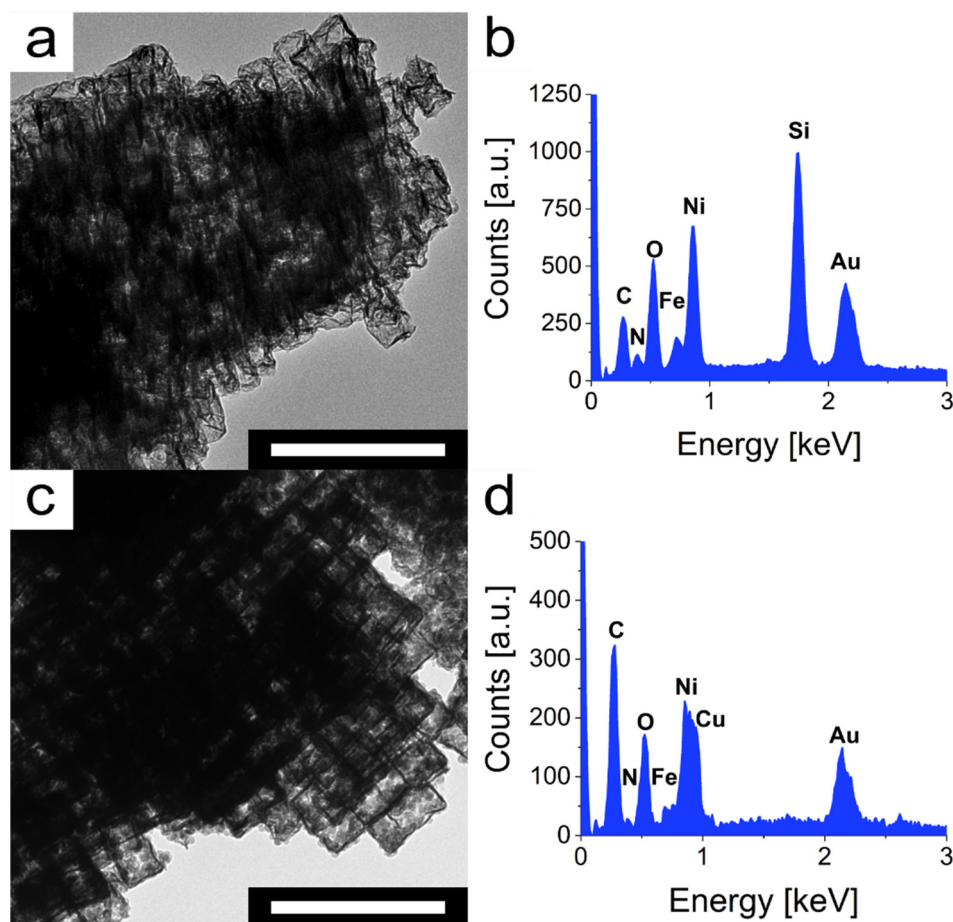
Figure 6. Analysis of the mesoframes morphology and composition after catalysis. (a) TEM micrograph of the mesoframes after rhodamine-B removal. (b) EDS spectrum of mesoframes after the catalysis. Reaction conditions: [Rhodamine-B] = 10.0 mg L -1 , V = 100 mL, T = 25 °C, pH = 5, [Mesoframe] = 0.10 g L -1 , [PMS] = 0.30 g L -1 . (c) TEM micrographs of the mesoframes after bisphenol-A catalysis. (d) Corresponding EDS spectrum of mesoframes after the bisphenol-A catalysis (Copper signal obtained from analyzed TEM mesh). Reaction conditions: [Bisphenol-A] = 40.0 mg L -1 , V = 100 mL, T = 25 °C, pH = 7, [Mesoframe] = 0.20 g L -1 , [PMS] = 0.20 g L -1 . Scale bars: 500 nm.
