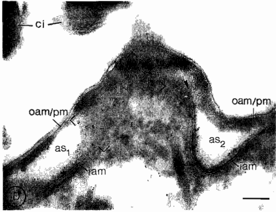
FIG. 16 A SERCA-type Ca^{2+} pump occurs in the alveolar sacs of Paramecium . Its gene has been cloned. The amino acid sequence derived for one of the transmembrane domains shown in (A) reveals wide variation between species. Because this region is reported to bind the inhibitor, thapsigargin, this wide aberration from the mammalian form in Paramecium and some of the Apicomplexa may explain the low sensitivity to this drug. The framed region has been used to prepare ABs. Their application in Western blots (B) to pellicles (surface complex), alveolar sacs (as), microsomes (mi), plasma membrane fractions (pm), and cilia (ci) shows enrichment of this pump (106 kDa) in alveolar sacs. Immunolocalization in CLSM (C) or EM (D) analysis also shows the occurrence of the SERCA-type pump in alveolar sacs [patches in en face view (C), outlines in median view (C')], notably their inner membrane [using a SERCA-specific AB, as specified in Plattner et al. (1999), which also recognizes SERCA in nearby ER]. Note the absence of gold label from the plasma membrane (pm) and the outer alveolar sac membrane (oam), in contrast to particularly heavy labeling at a site where an inner alveolar sac membrane (iam) is met in a tangential section ( as_1 ), and also the occurrence of label along a cross-cut inner alveolar sac membrane (iam in as_2 ), and also the occurrence of label along a cross-cut inner alveolar sac membrane (iam in as_2 ). Bars = 10 \mu m (C), 0.1 \mu m (D). (A-C) from Hauser et al. (1998); (D) from Plattner et al. (1999).
